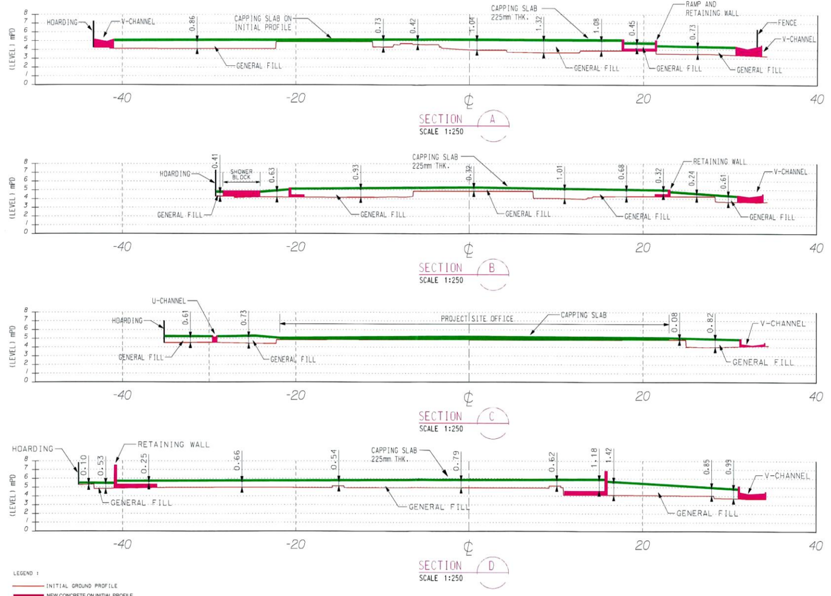
Figure 17: Mitigation Design at Works Area B 圖 17: 乙施工區的緩解設計
