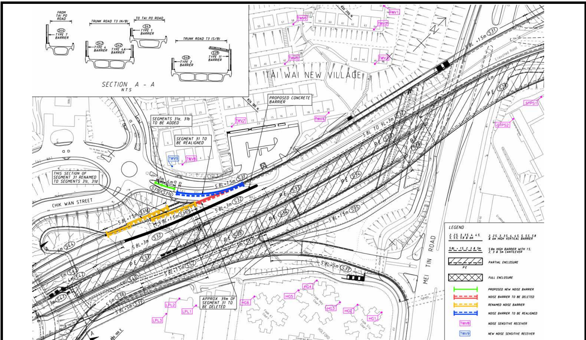
Figure 12 : Details of Noise Barriers segment nos. S31,S31a,S31b,S31c and S31d near Tai Wai New Village (Reproduced from Drawing No.T3/SSK5223A submitted under the Application for Variation of Environmental Permit (Application No.: VEP-242/2007))
