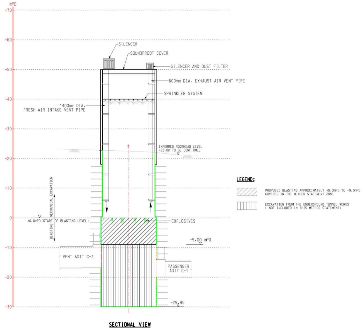
SECTIONAL VIEW
