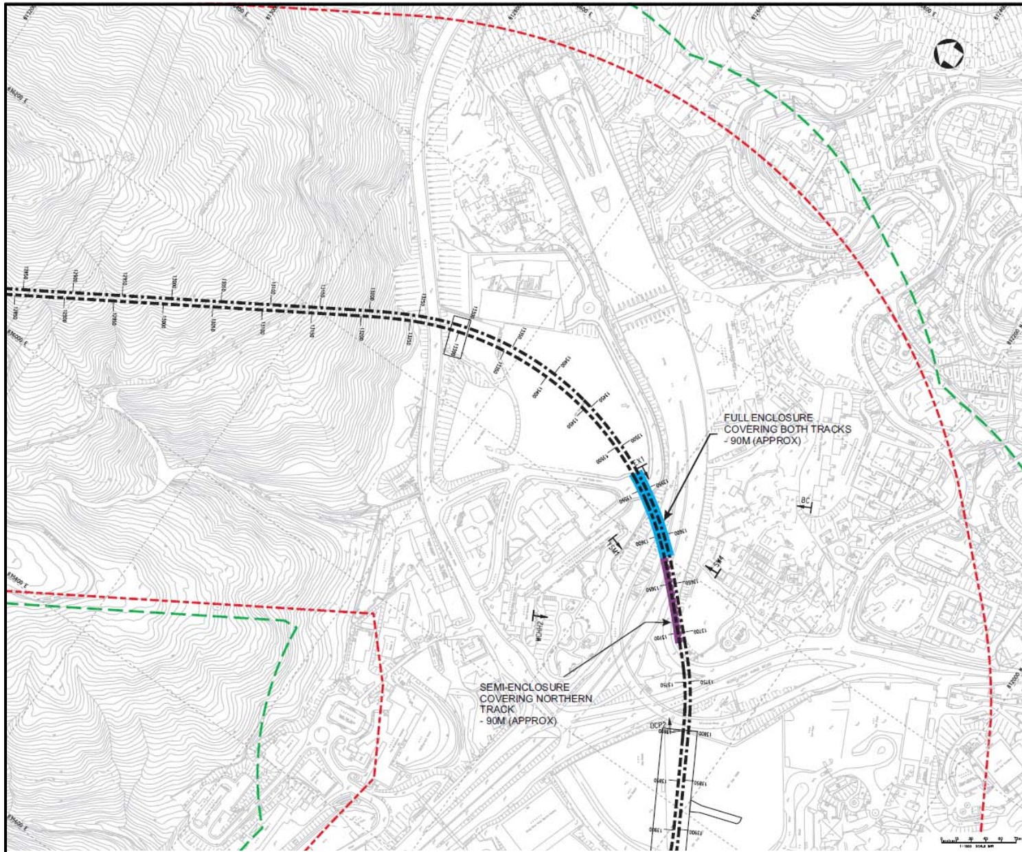
Figure 11: Mitigation Measures for Operational Air-Borne Noise 圖 11: 營辦期間的空氣傳導噪音緩解措施
