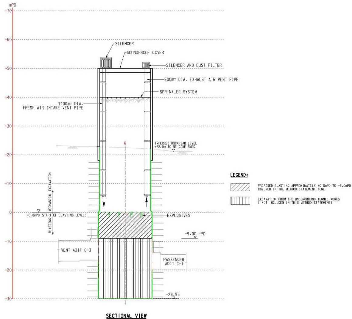
Figure 11: Mitigation Measures for Blasting at Works Area M3
