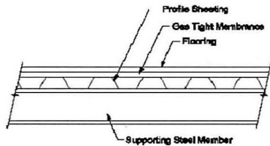
Detail A 1:30
