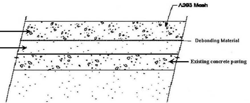
Detail B 1:30
