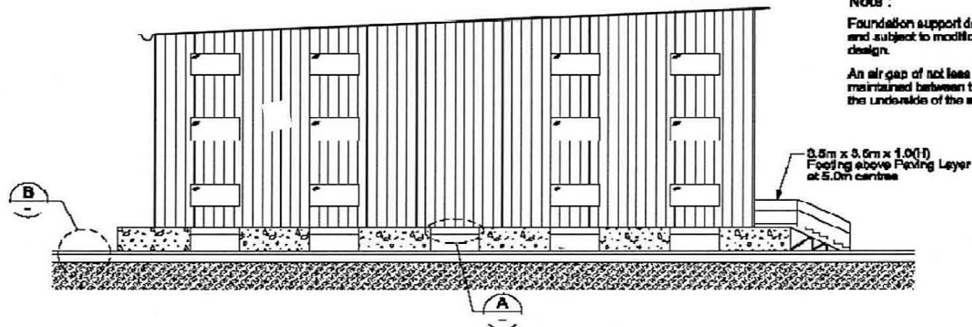
Figure 13: Mitigation Design at Works Area B
