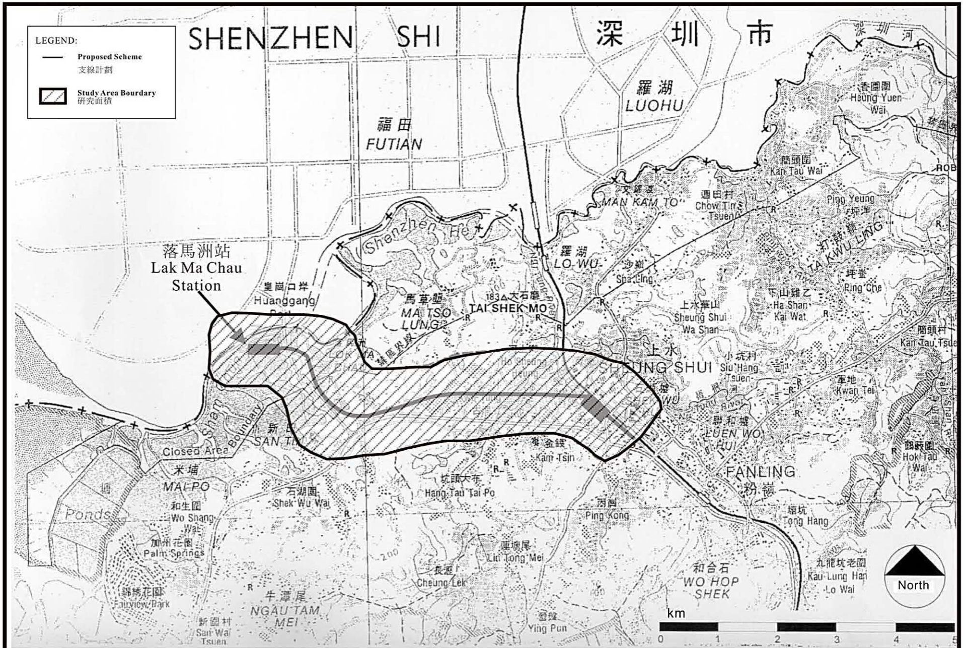
Sheung Shui to Lok Ma Chau Spur Line (上水至落馬洲支線) Figure 1A - Location of the Project 圖一A - 上水至落馬洲支線位置圖 (Reproduced from Drawing No.: 12.1 of (Volume 5 of 5) of the EIA Report (Register No.: AEIAR-052/2002) 摘自環評報告第五冊圖 12.1 (登記冊編號: AEIAR-052/2002)
