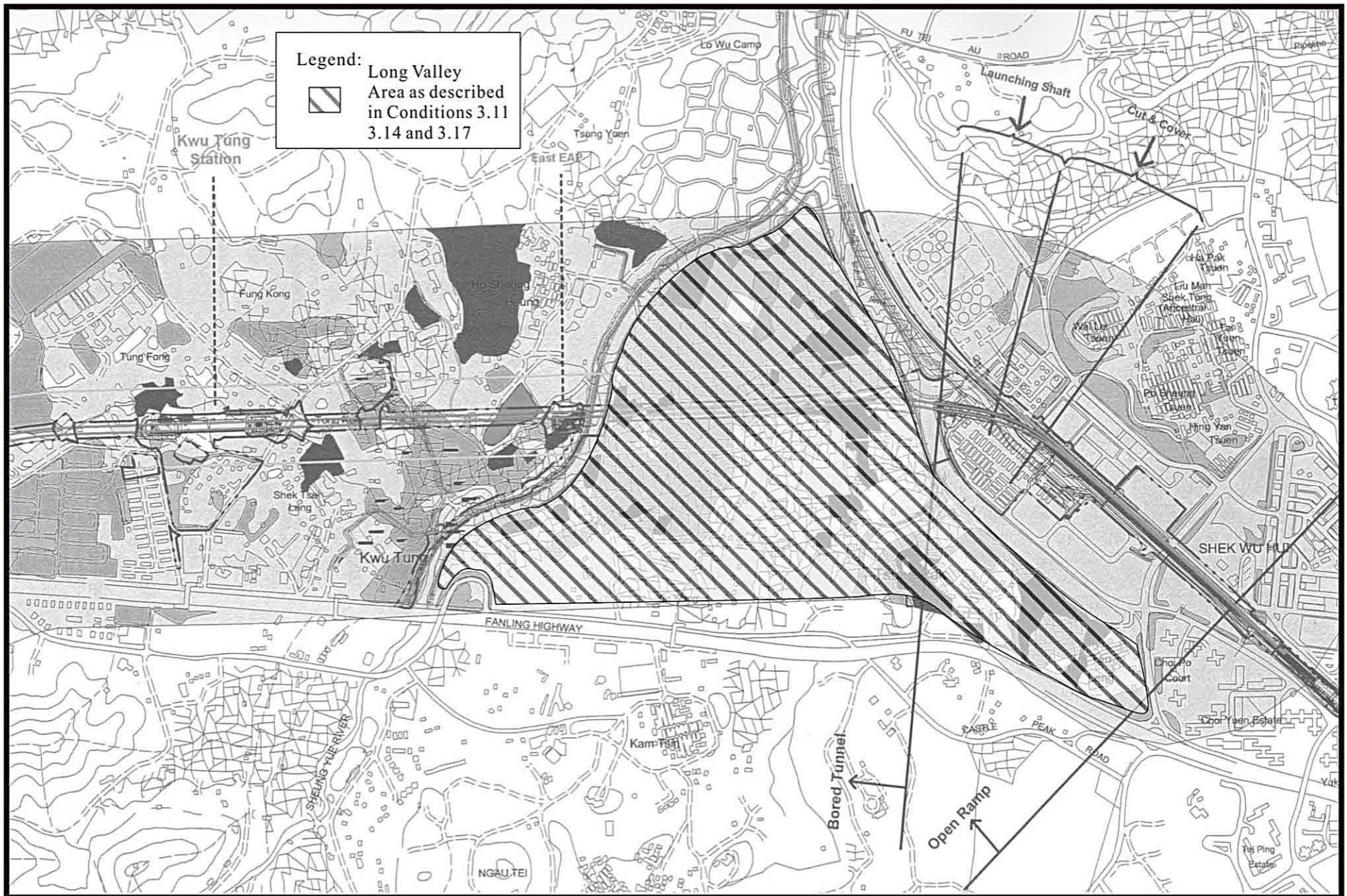
Figure 2 - Sheung Shui to Lok Ma Chau Spur Line (上水至落馬洲支線) 圖二 - 塲原位置圖 (Reproduced from Drawing No.: 4.1b (Volume 5 of 5) of the EIA Report (Register No.: AEIAR-052/2002) 摘自環評報告第五冊圖4.1b(登記冊編號:AEIAR-052/2002)
