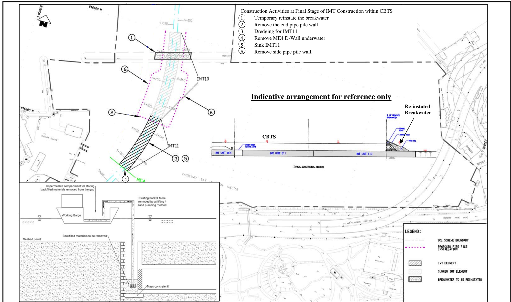
Figure 10: Final Stage of IMT Construction at CBTS
