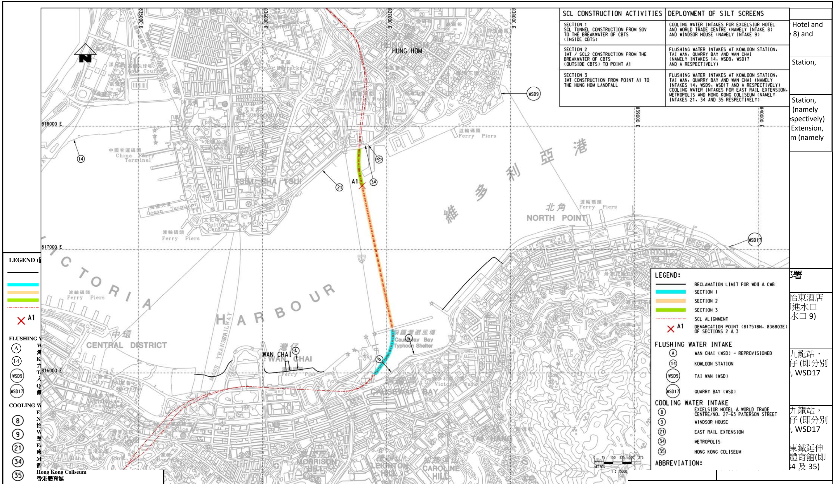
Figure 4: Sections of SCL Construction Activities and the Locations of Cooling Water Intake and WSD Flushing Water Intake
