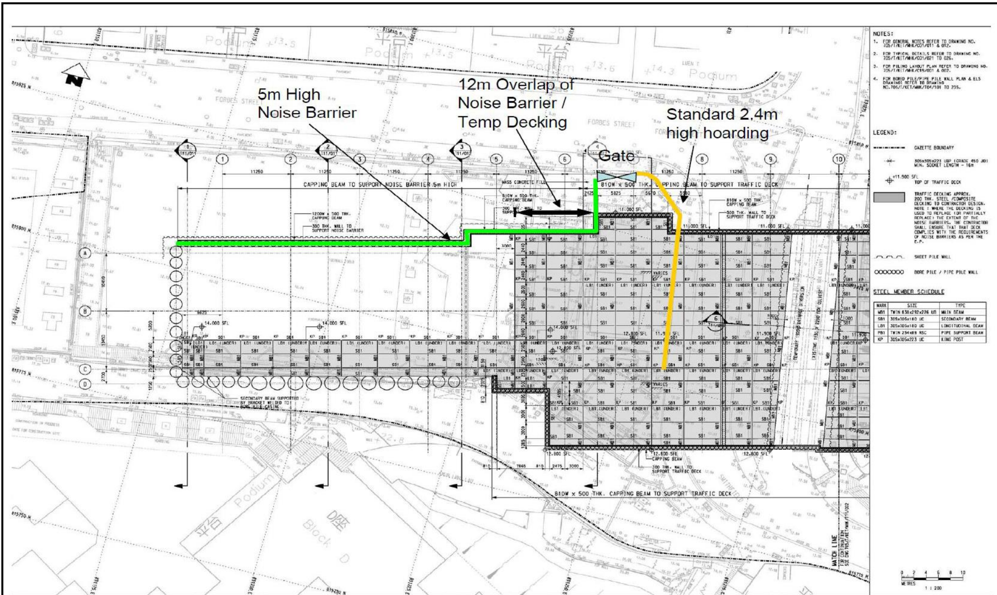
Figure :: Approximate Extend of Decking at Works Area C 圖 :: 施工區丙的大概鋪蓋範圍
