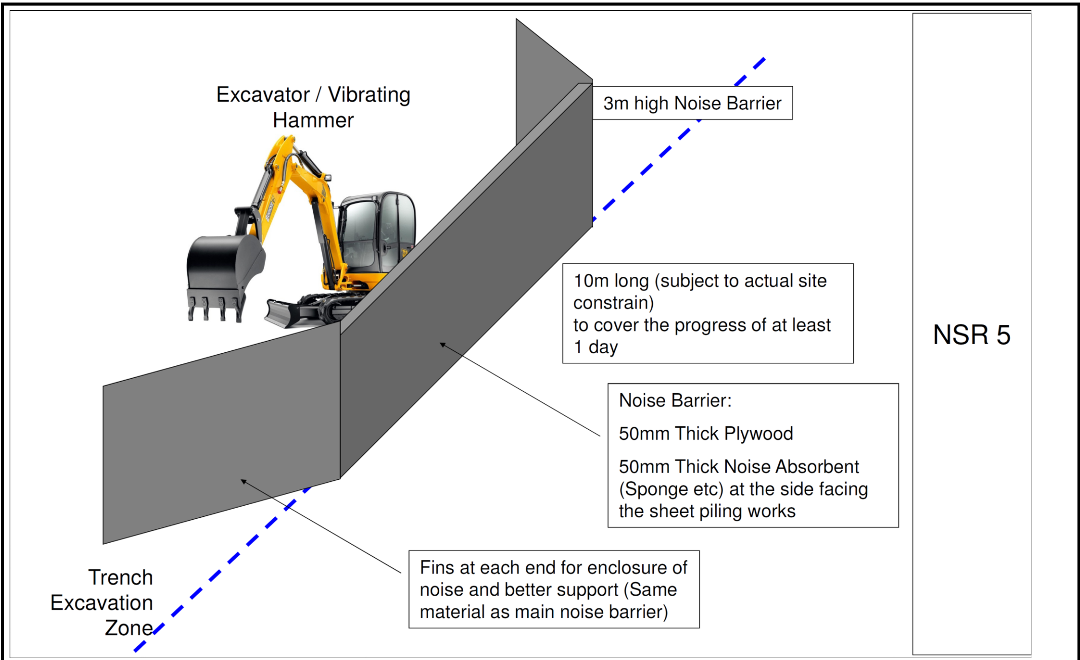
Figure 6 : Noise Barrier design
