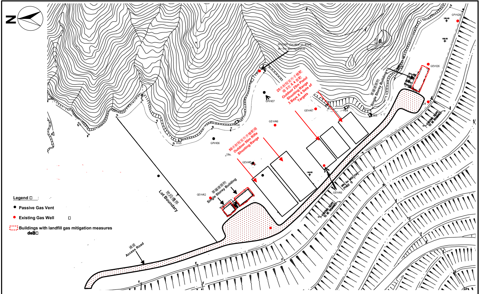
Figure 3 - Layout Plan of the Shooting Range
