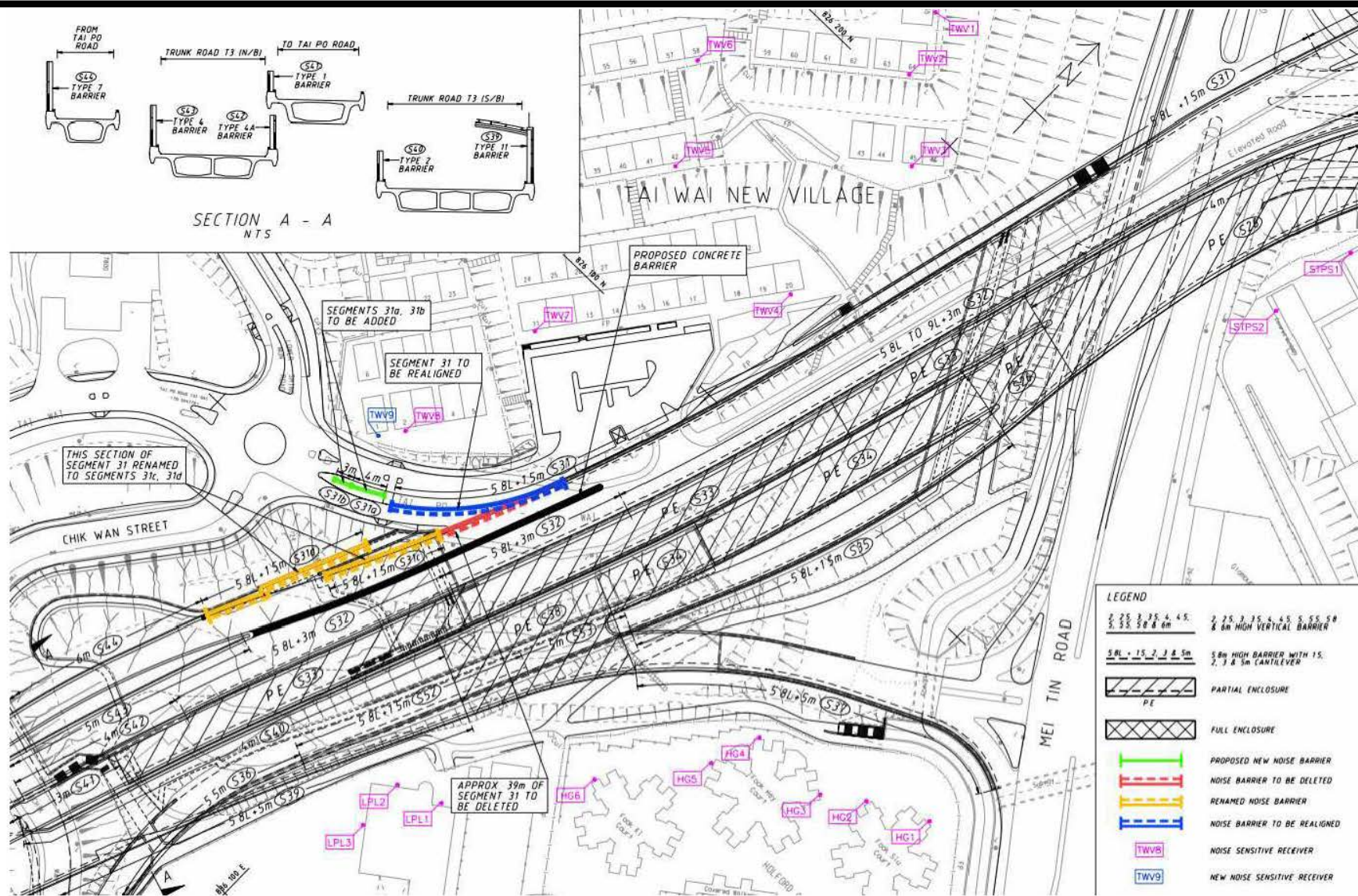
Figure 12 : Details of Noise Barriers segment nos. S31,S31a,S31b,S31c and S31d near Tai Wai New Village (Reproduced from Drawing No.T3/SSK5223A submitted under the Application for Variation of Environmental Permit (Application No.: VEP-242/2007))
