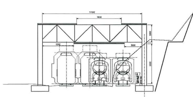
TYPICAL CROSS SECTION B
