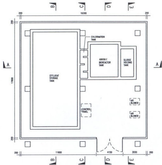
SECTIONAL PLAN
