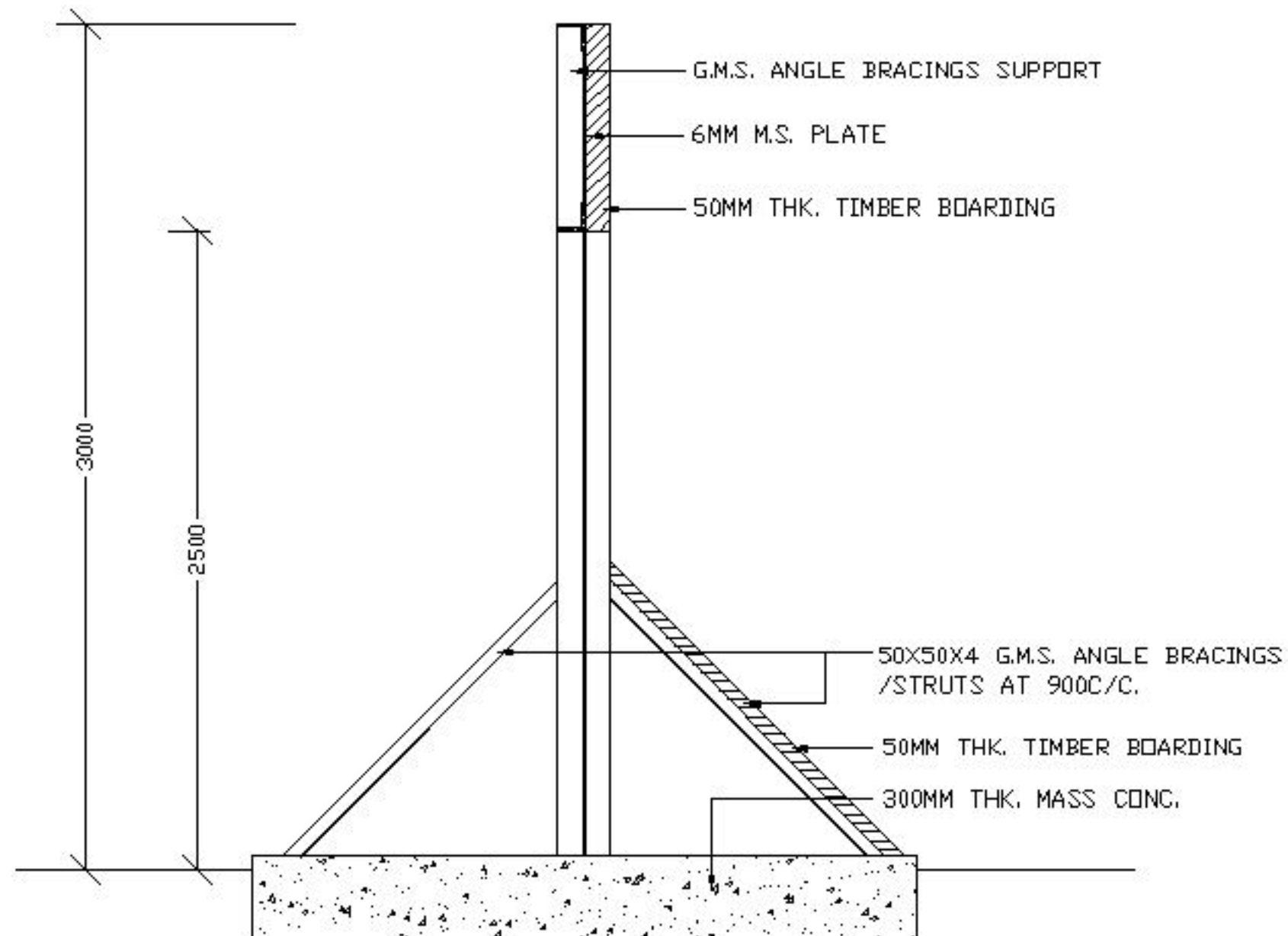
2 D-02 TYPICAL DETAIL OF SHOOTING RANGE OVERHEAD ARCH
