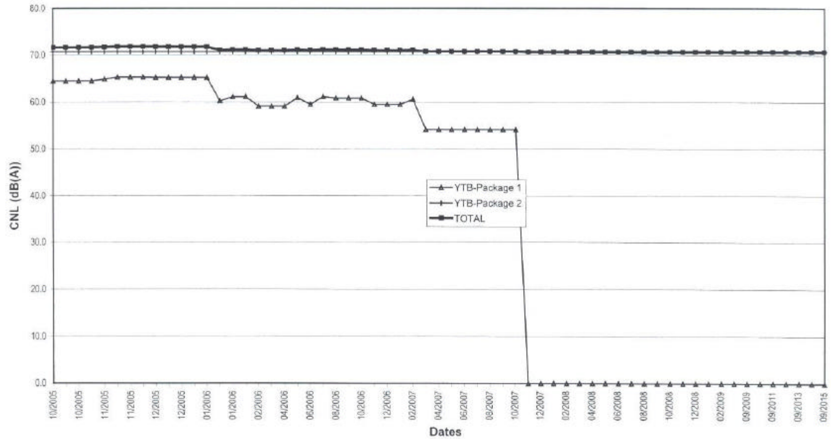
Figure A6.9 Predicted Cumulative Construction Noise Levels at "REHC3"
