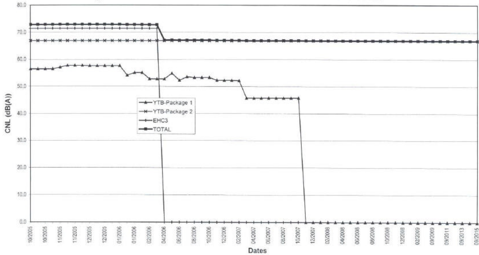
Figure A6.1 Predicted Cumulative Construction Noise Levels at "RYTE1"
