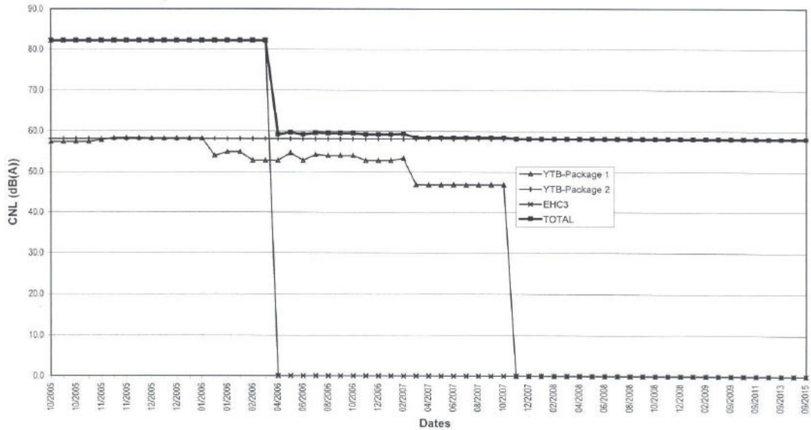
Figure A6.10 Predicted Cumulative Construction Noise Levels at "RSCH1"
