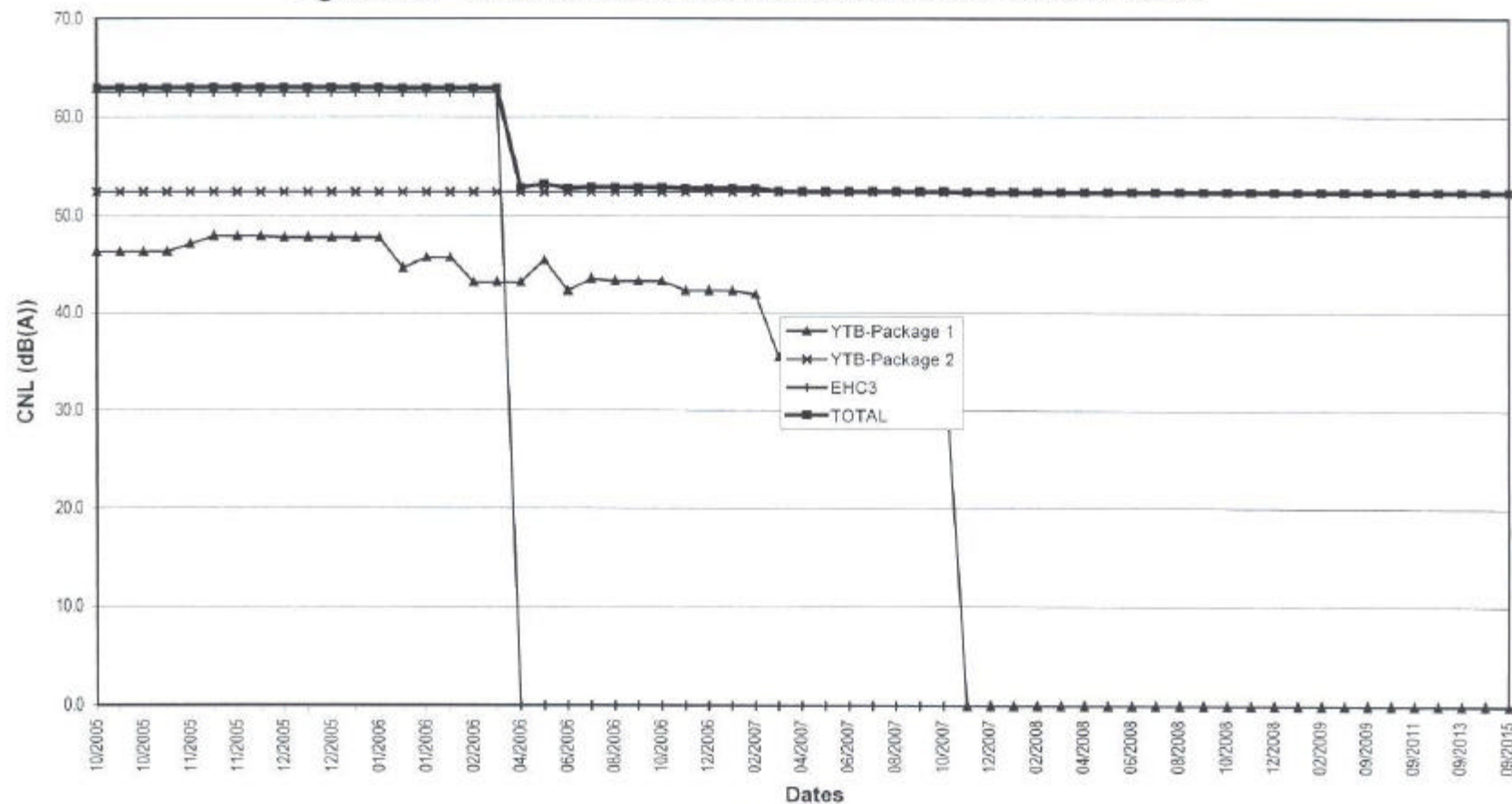
Figure A6.5 Predicted Cumulative Construction Noise Levels at "RYCT"
