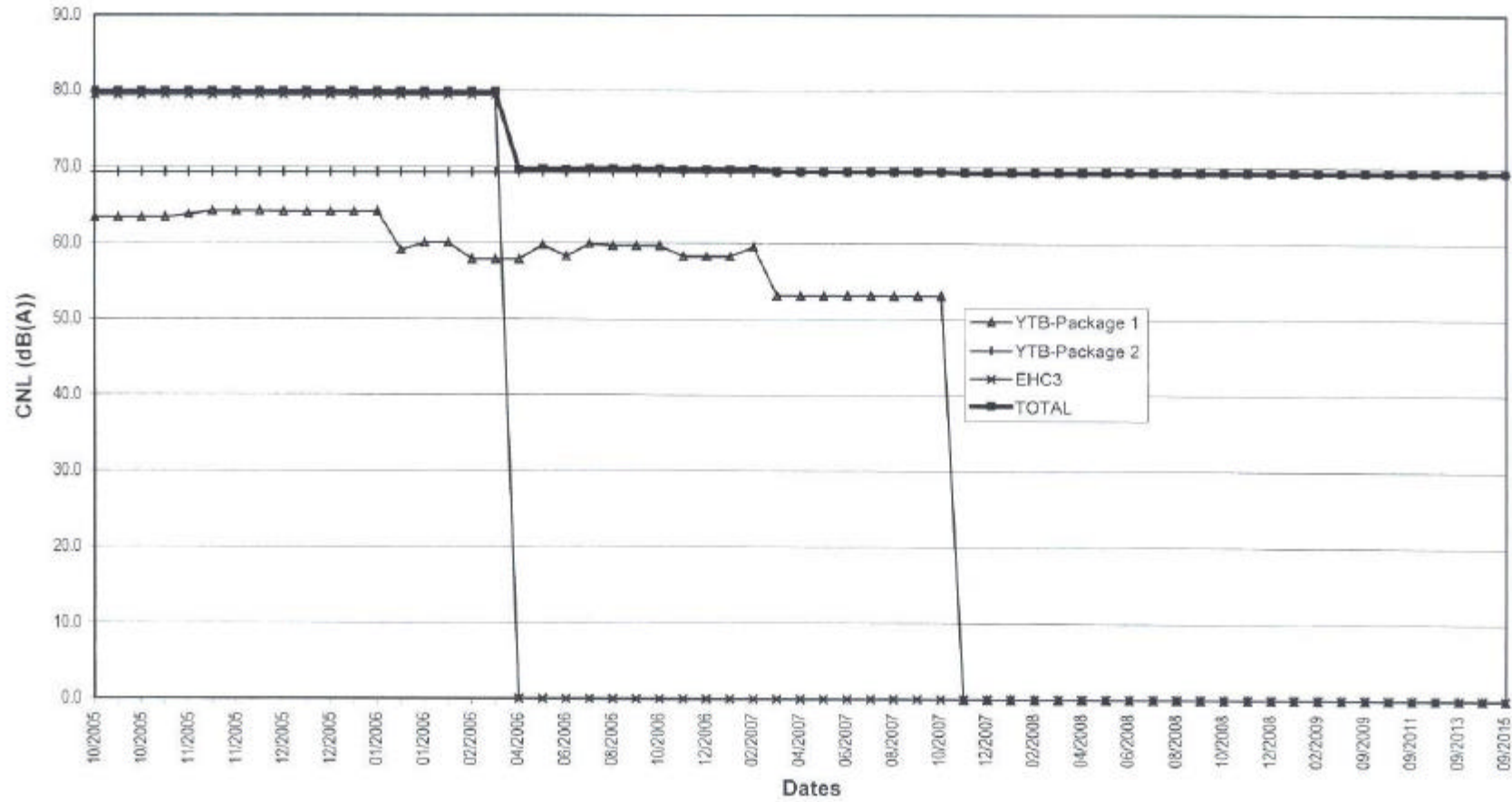
Figure A6.12 Predicted Cumulative Construction Noise Levels at "RSCH3"
