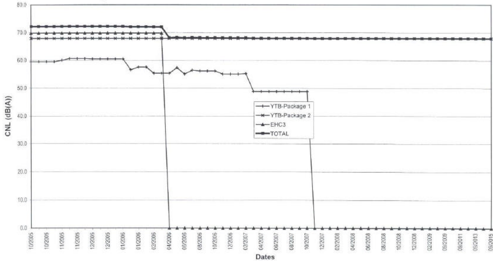
Figure A6.4 Predicted Cumulative Construction Noise Levels at "RYTE5"
