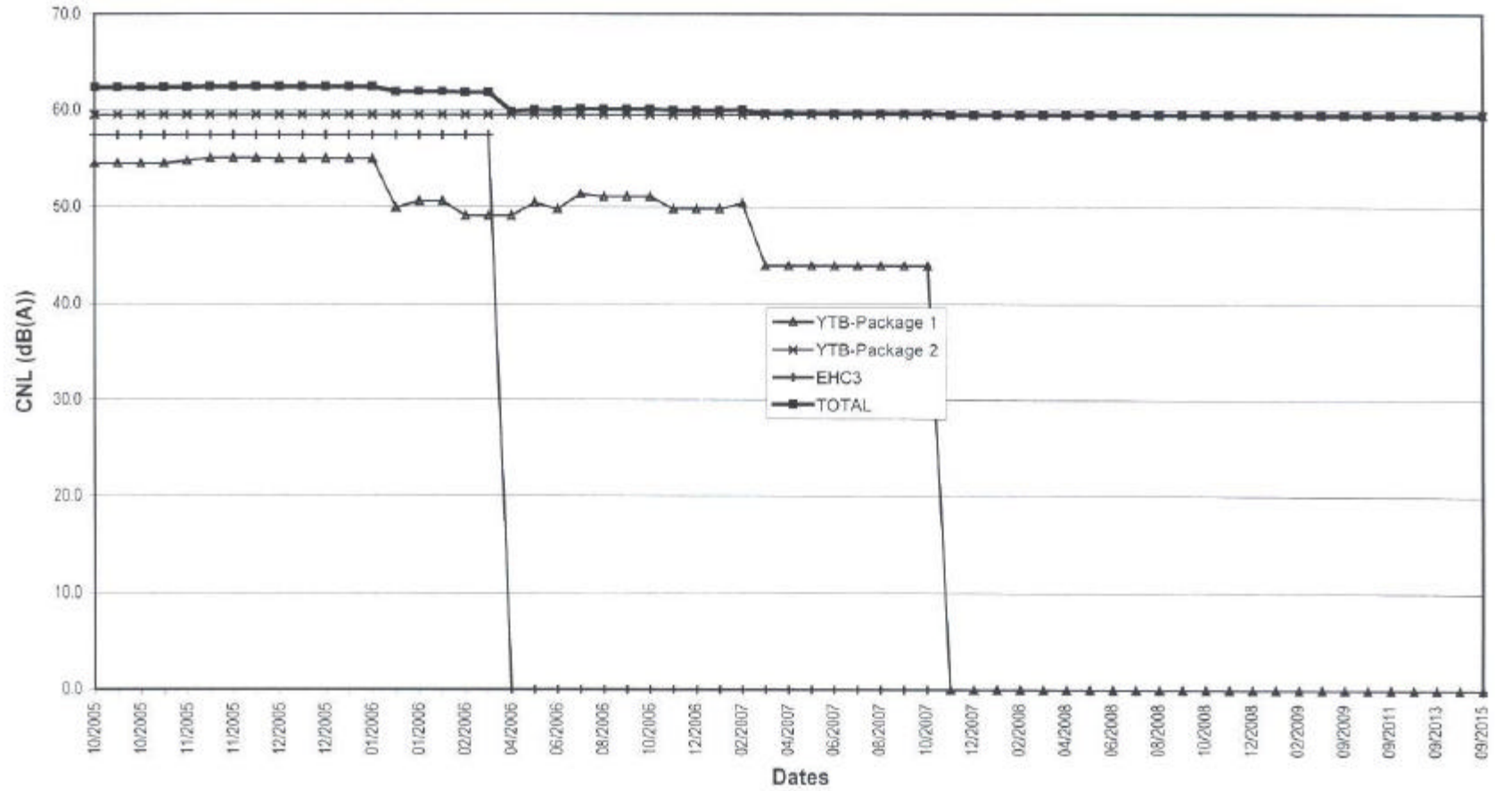
Figure A6.6 Predicted Cumulative Construction Noise Levels at "RCKL"
