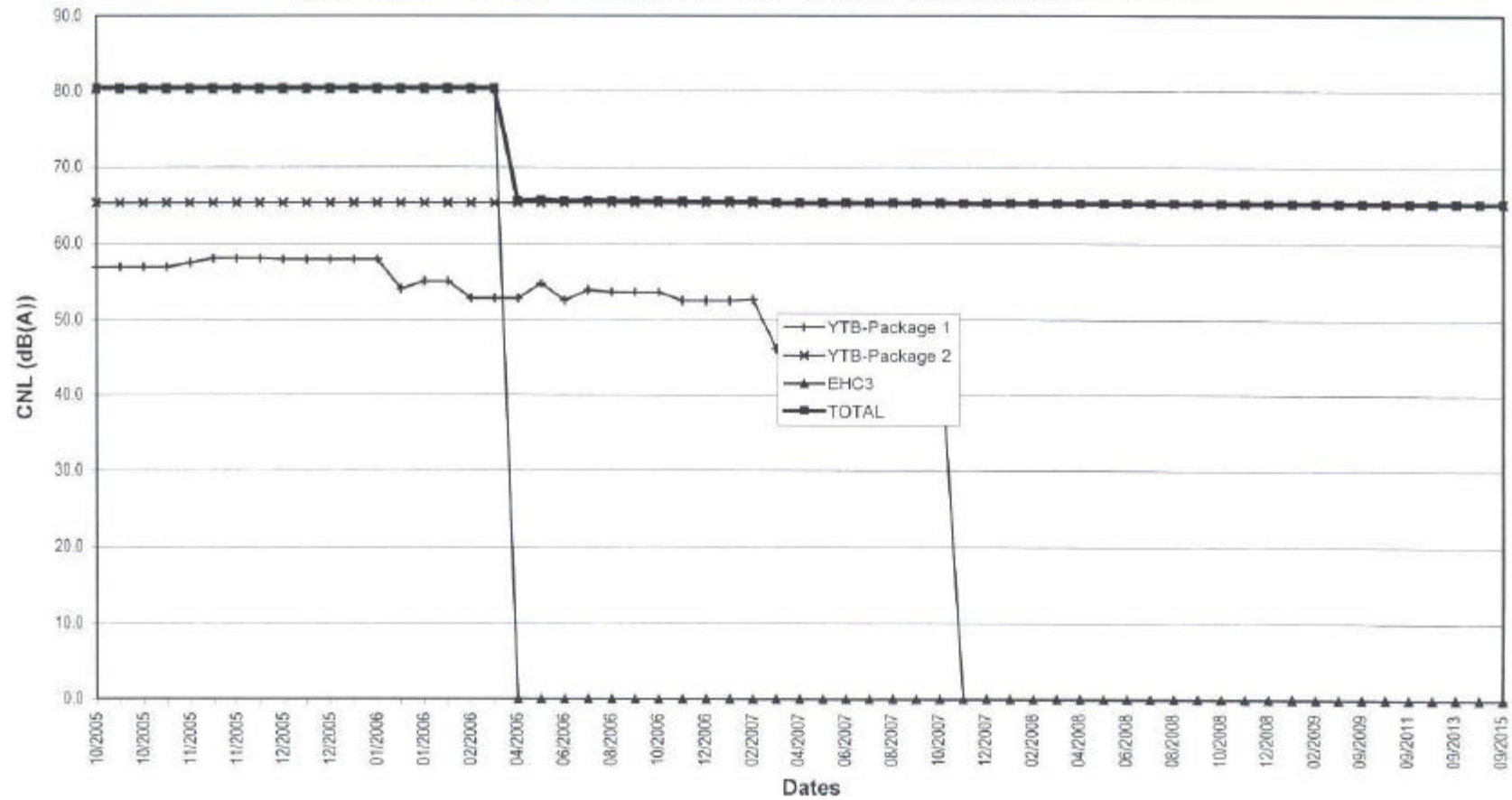
Figure A6.2 Predicted Cumulative Construction Noise Levels at "RYTE2"
