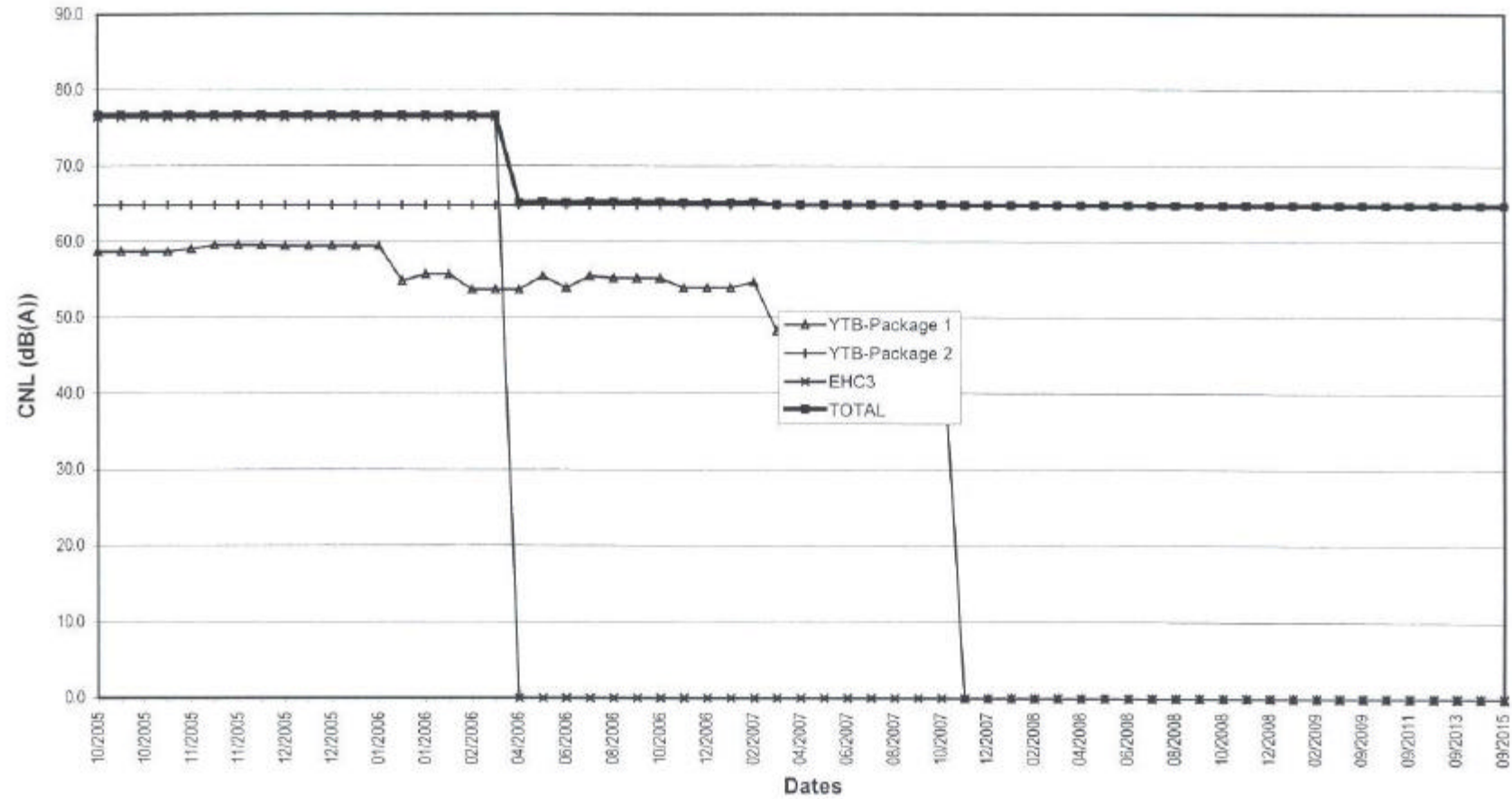
Figure A6.7 Predicted Cumulative Construction Noise Levels at "REHC1"
