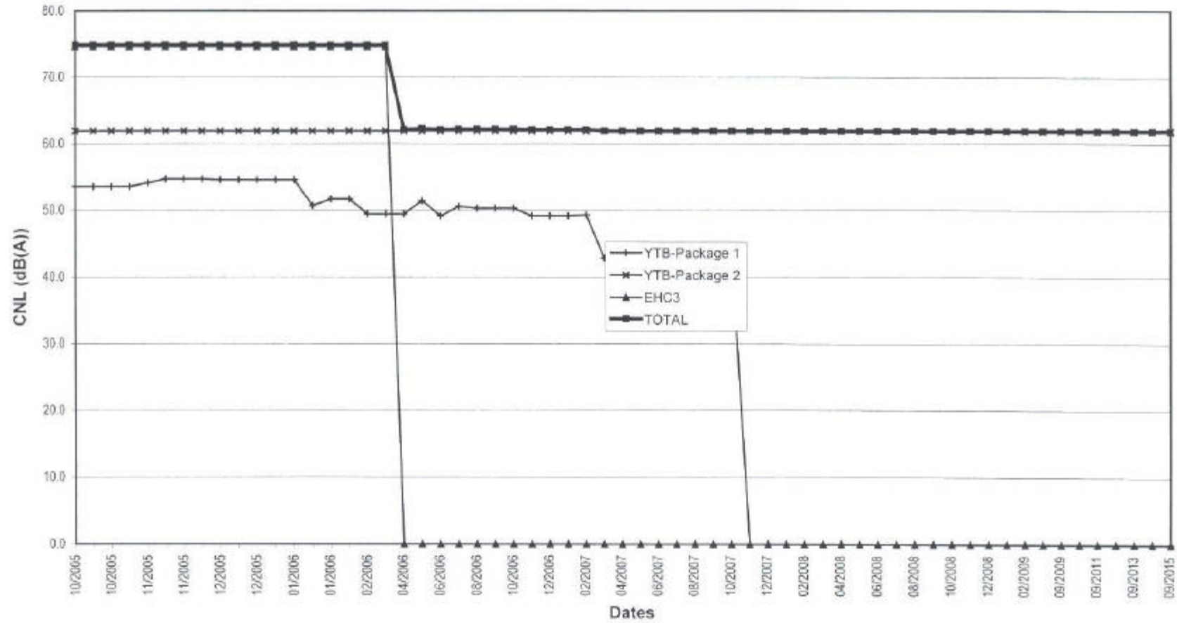
Figure A6.3 Predicted Cumulative Construction Noise Levels at "RYTE3"
