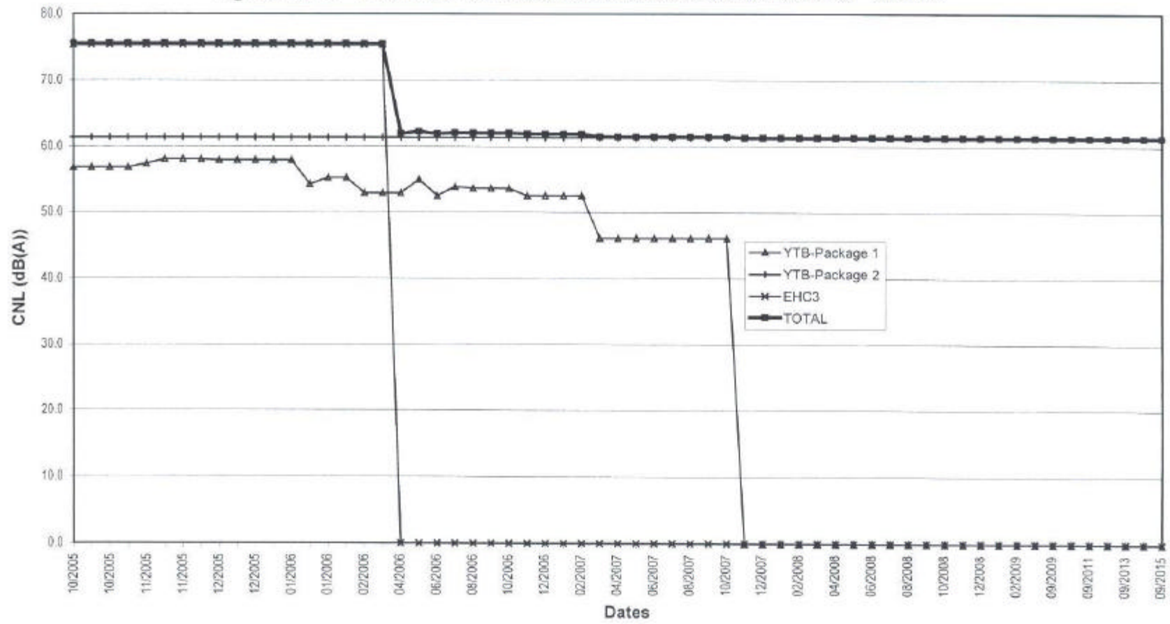
Figure A6.11 Predicted Cumulative Construction Noise Levels at "RSCH2"
