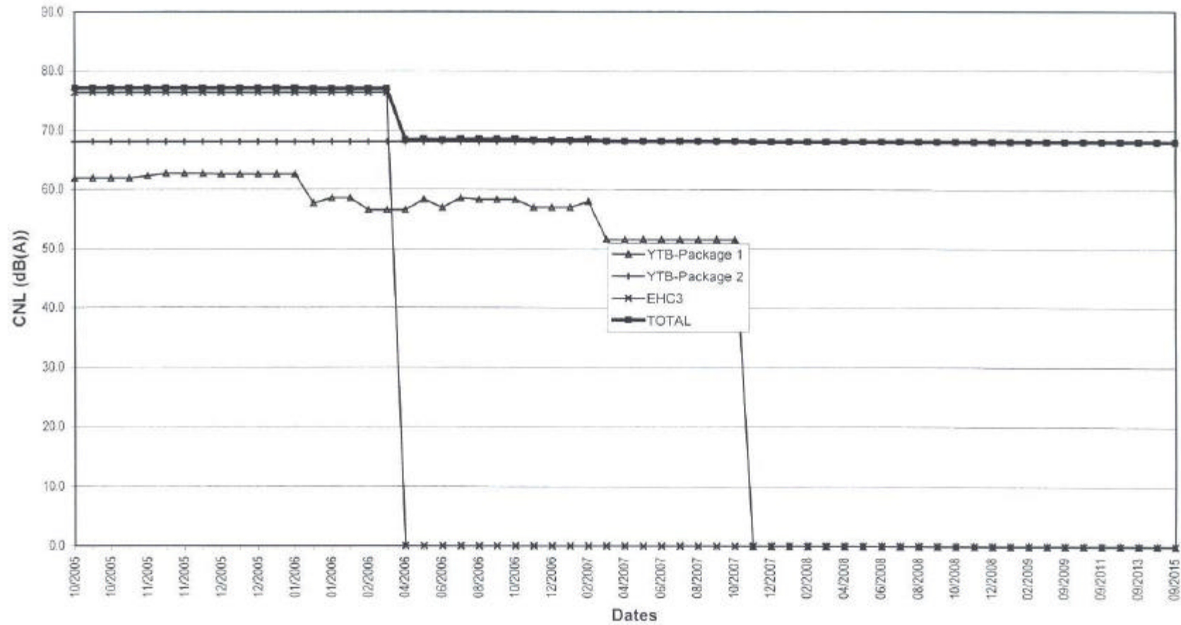
Figure A6.8 Predicted Cumulative Construction Noise Levels at "REHC2"
