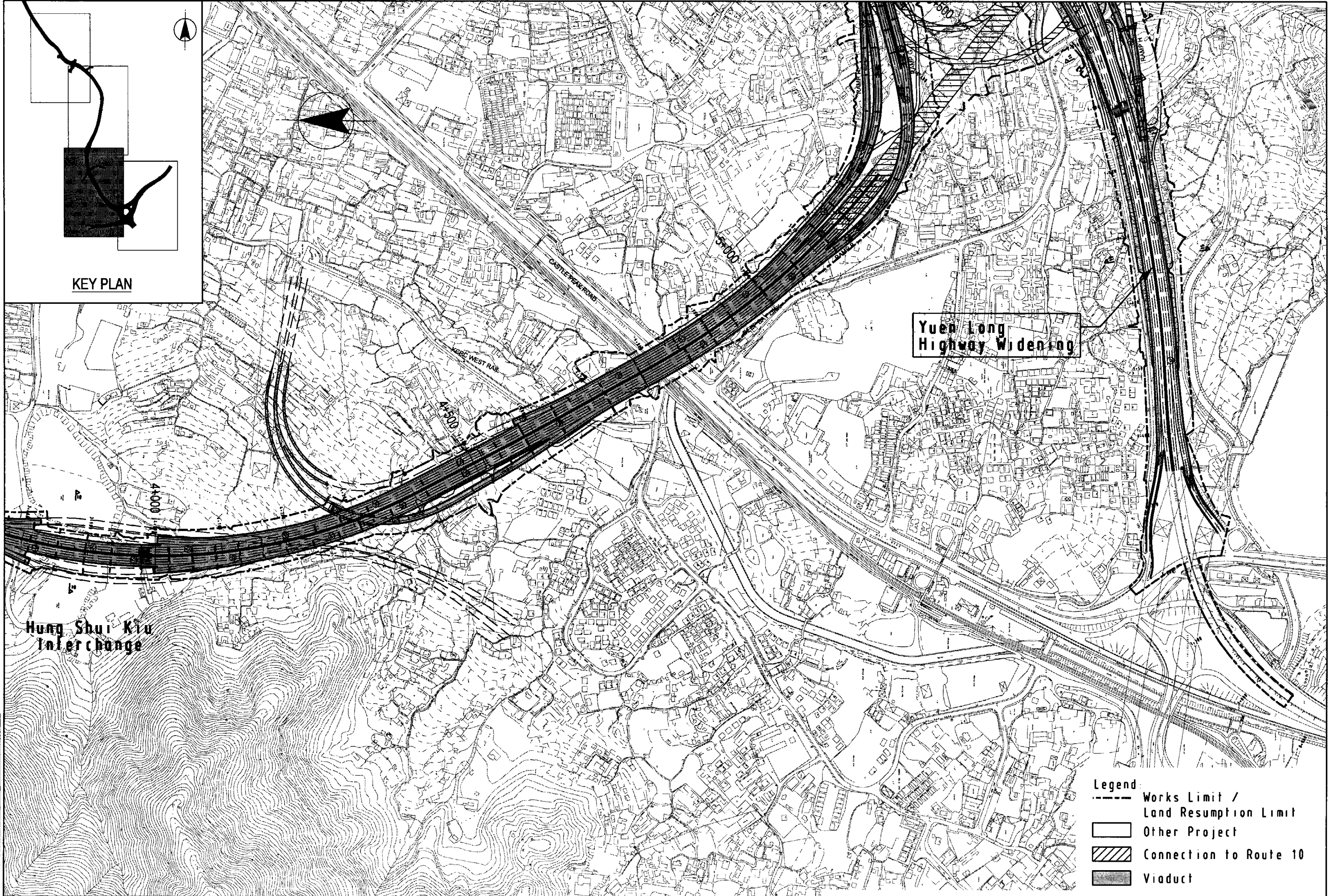
Figure 1.1C Deep Bay Link General Layout Plan
