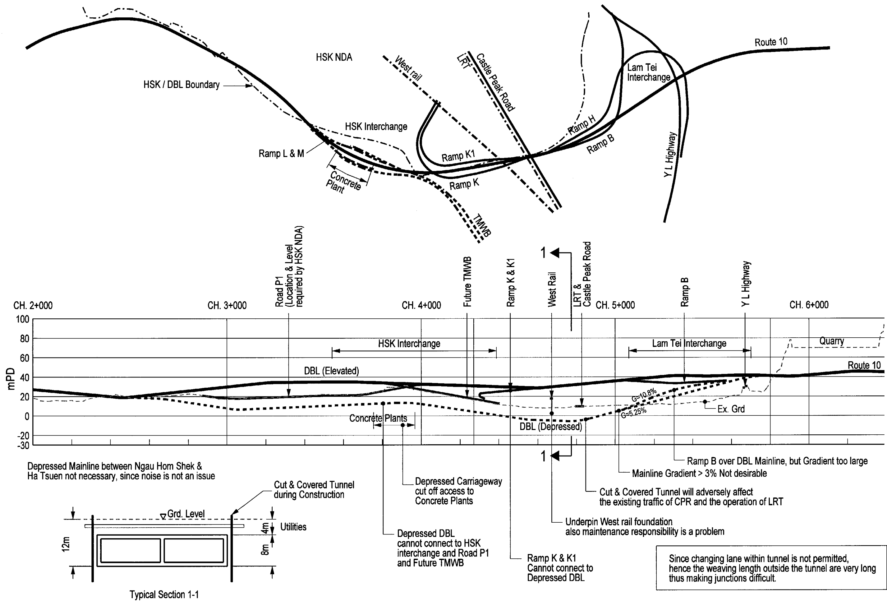
Figure 1.7 Depressed Alignment of Deep Bay Link
