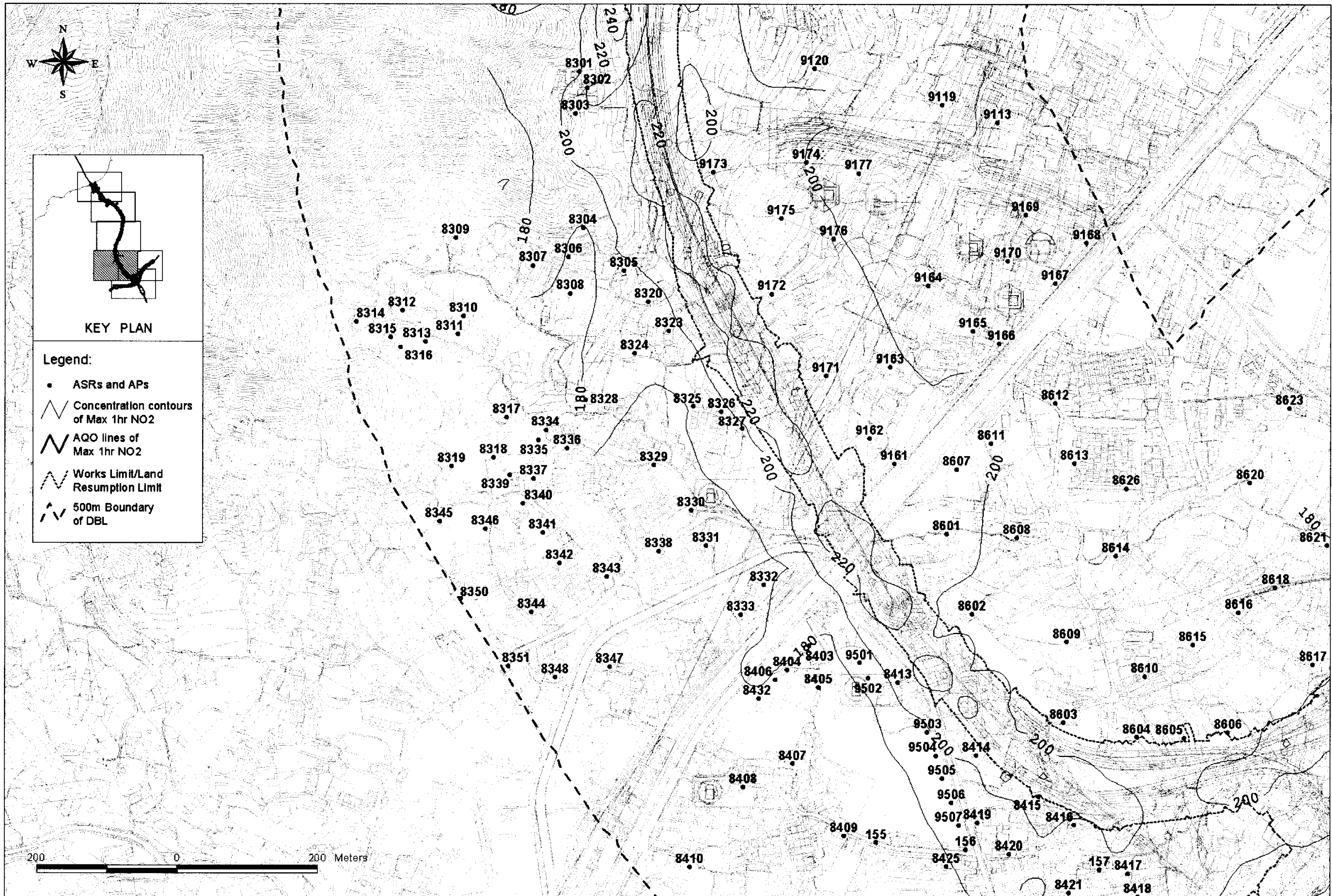
Figure 2.2D Concentration Contours of Predicted Worst-case 1-hour Average Nitrogen Dioxide Level at 1.5m Above Ground
