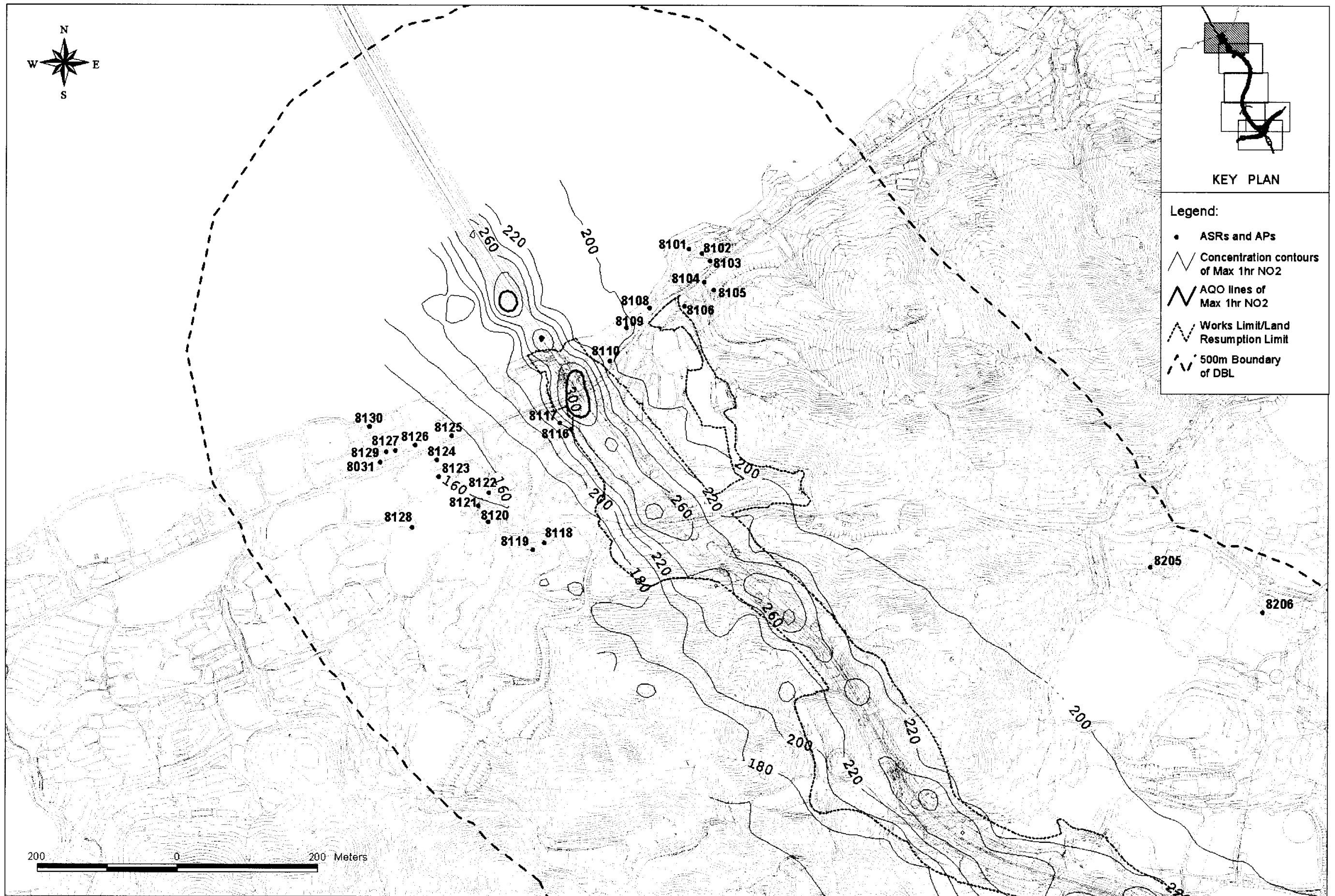
Figure 2.3A Concentration Contours of Predicted Worst-case 1-hour Average Nitrogen Dioxide Level at 10m Above Ground
