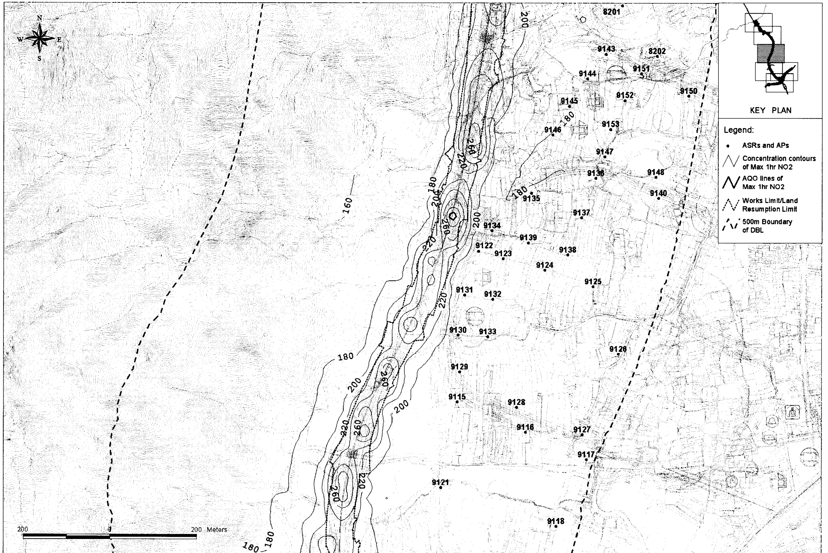
Figure 2.3C Concentration Contours of Predicted Worst-case 1-hour Average Nitrogen Dioxide Level at 10m Above Ground
