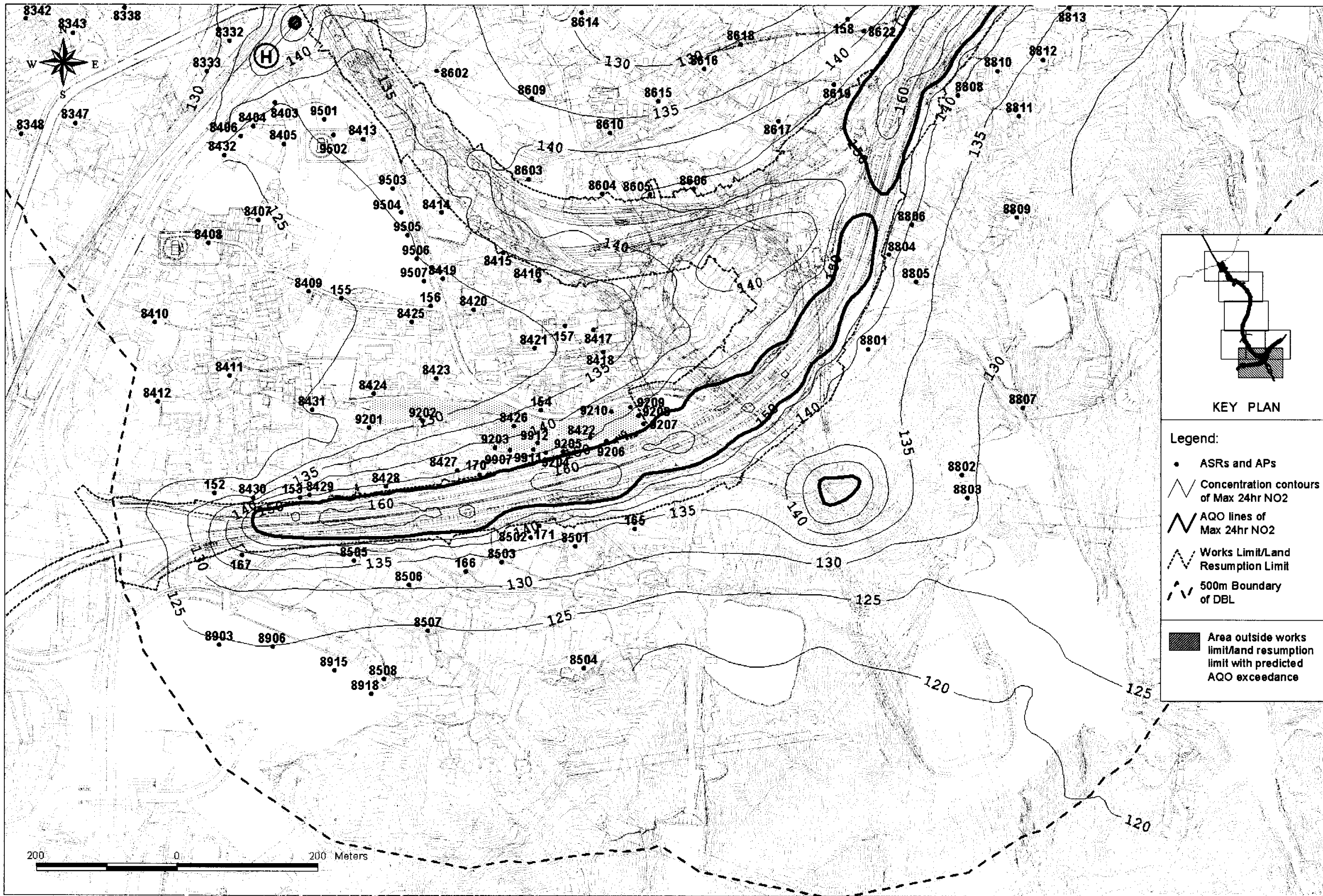
Figure 2.4F Concentration Contours of Predicted Worst-case 24-hour Average Nitrogen Dioxide Level at 1.5m Above Ground
