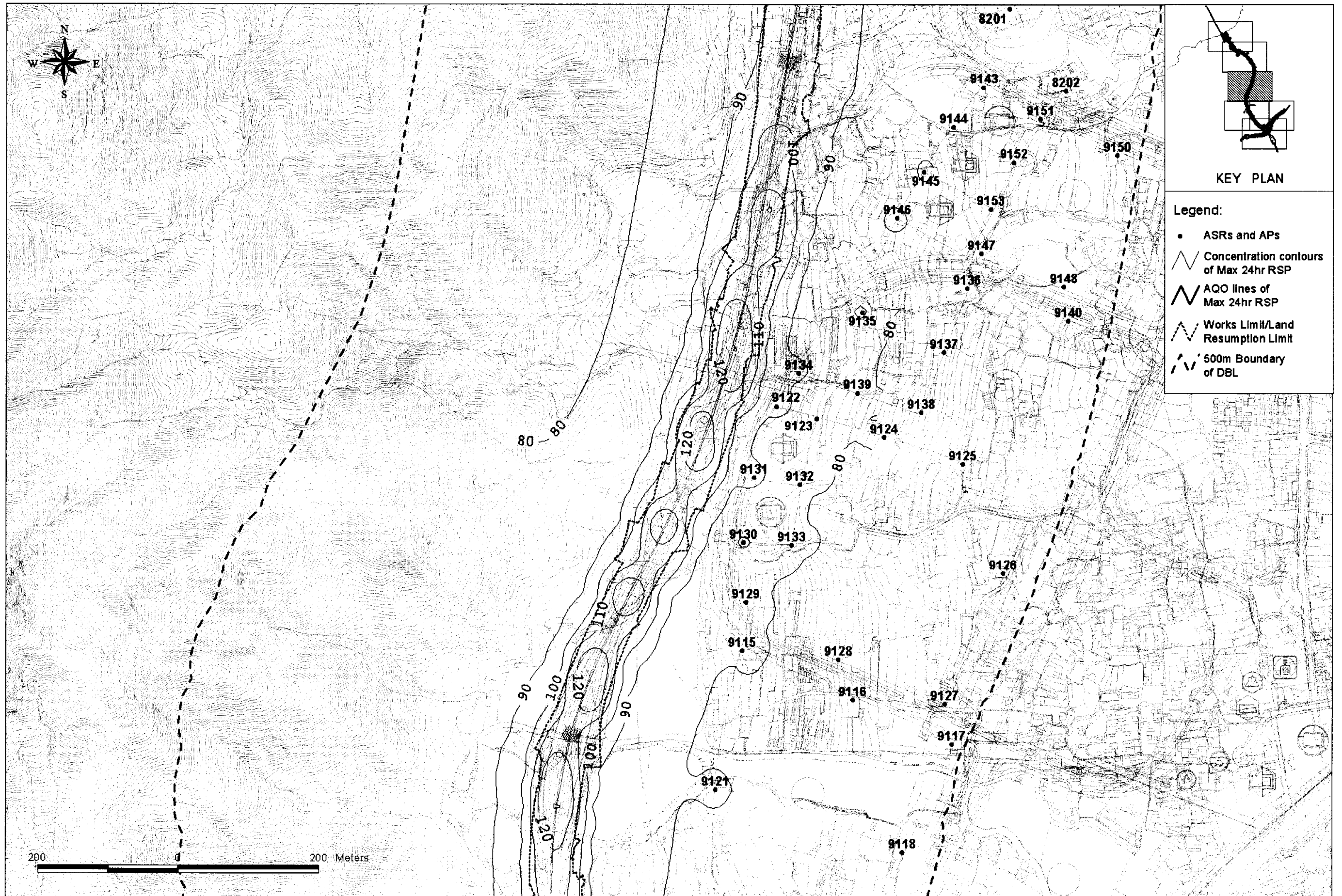
Figure 2.7C Concentration Contours of Predicted Worst-case 24-hour Average Respirable Suspended Particulates Level at 10m Above Ground
