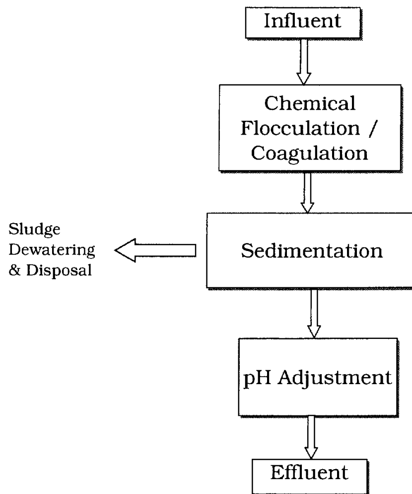
Figure 4.4 A Schematic Sketch of a Commercial Wastewater Treatment System and its Performance
