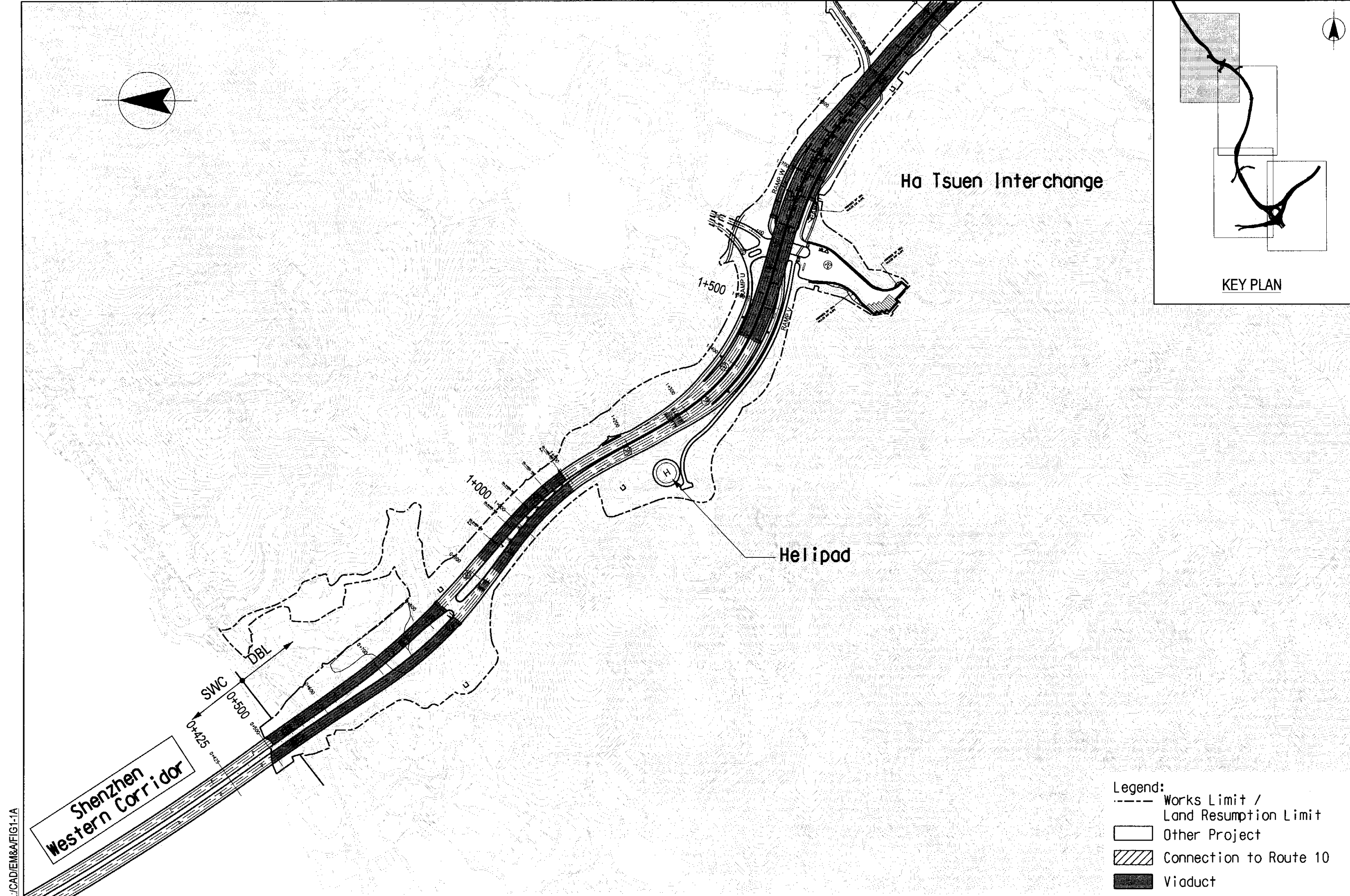
Figure 1.1A Proposed Deep Bay Link Alignment
