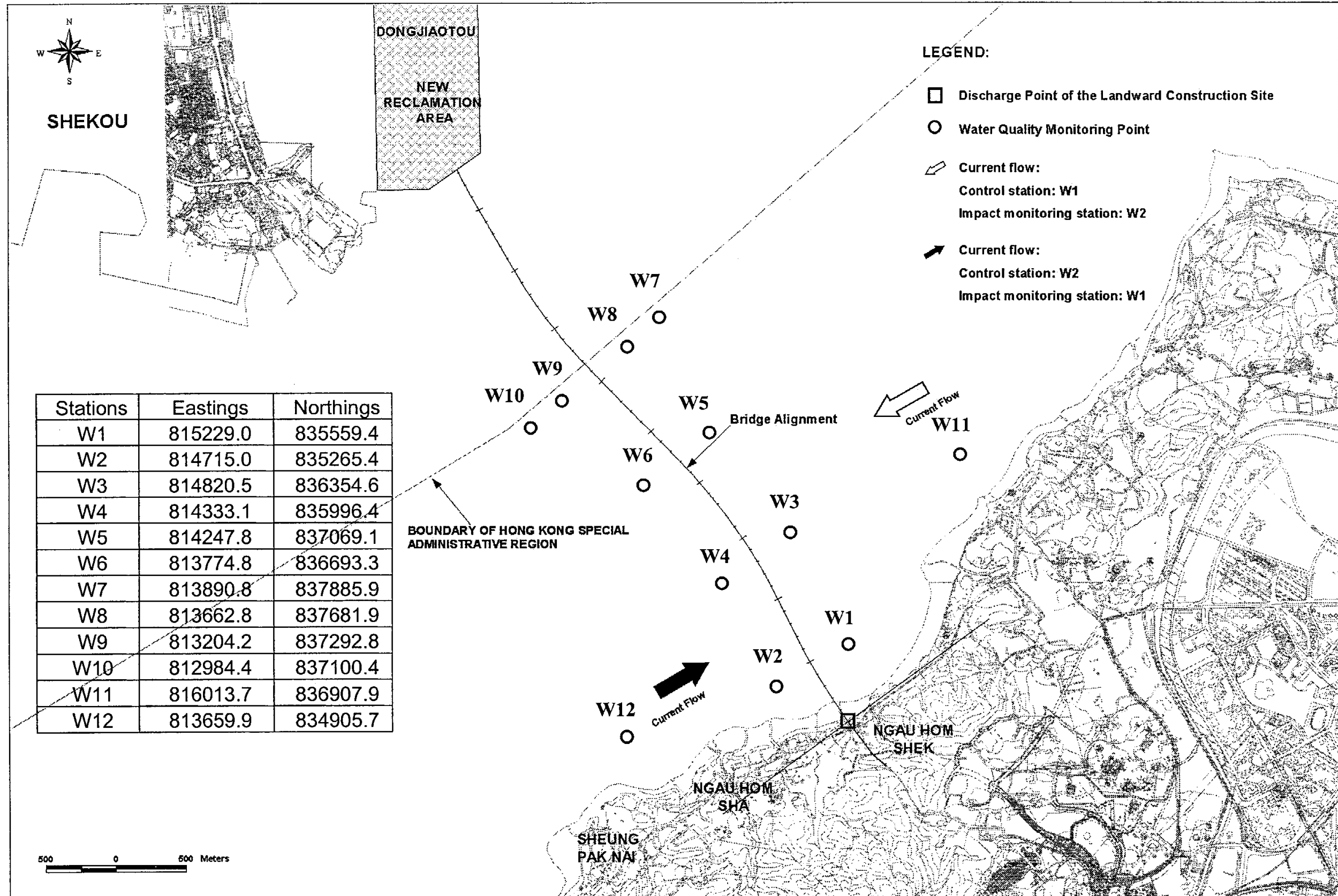
Figure 4.3 Water Monitoring Stations for SWC Project (W1 and W2 are common for DBL and SWC)
