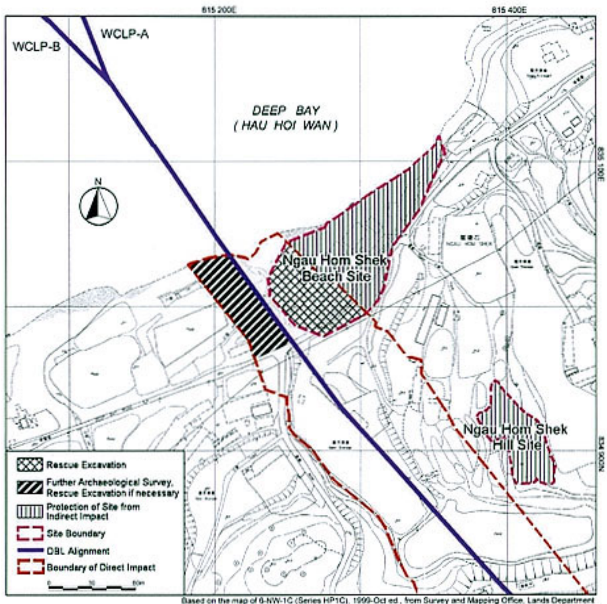
Figure 8.1 Plan of Mitigation Measures at Ngau Hom Shek
