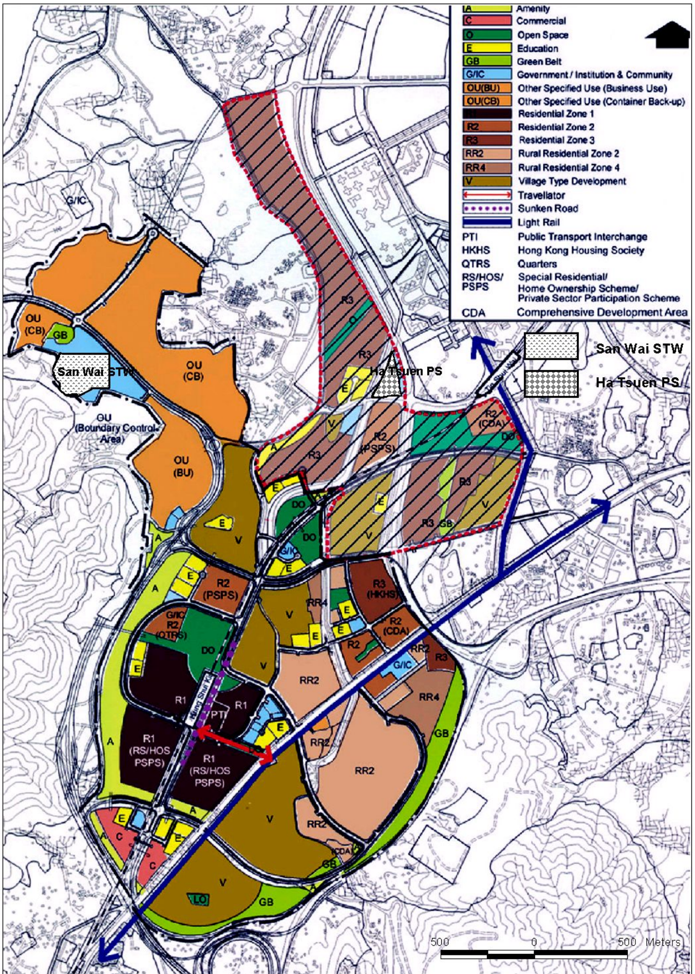
Figure 1.9 HSKND Recommended Outline Development Plan (RODP)
