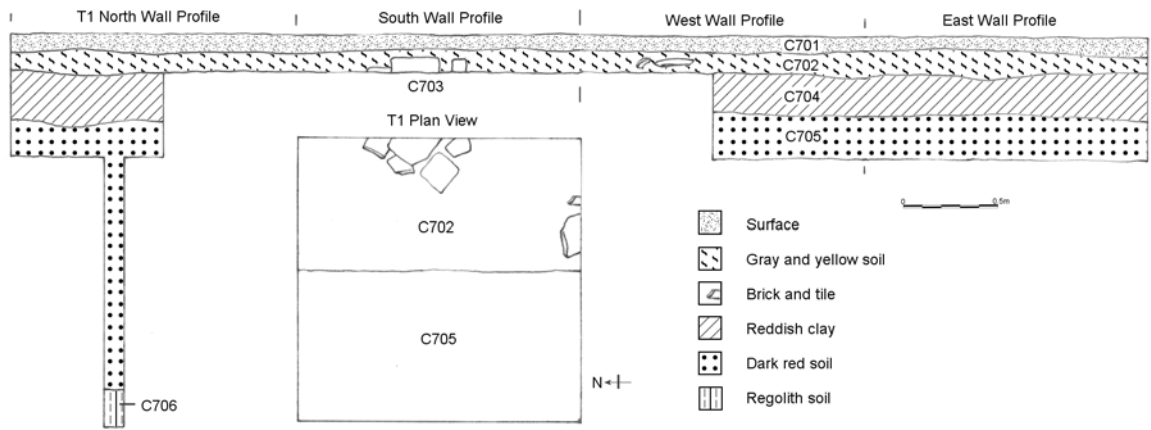
1. T1 Section and Plan View
