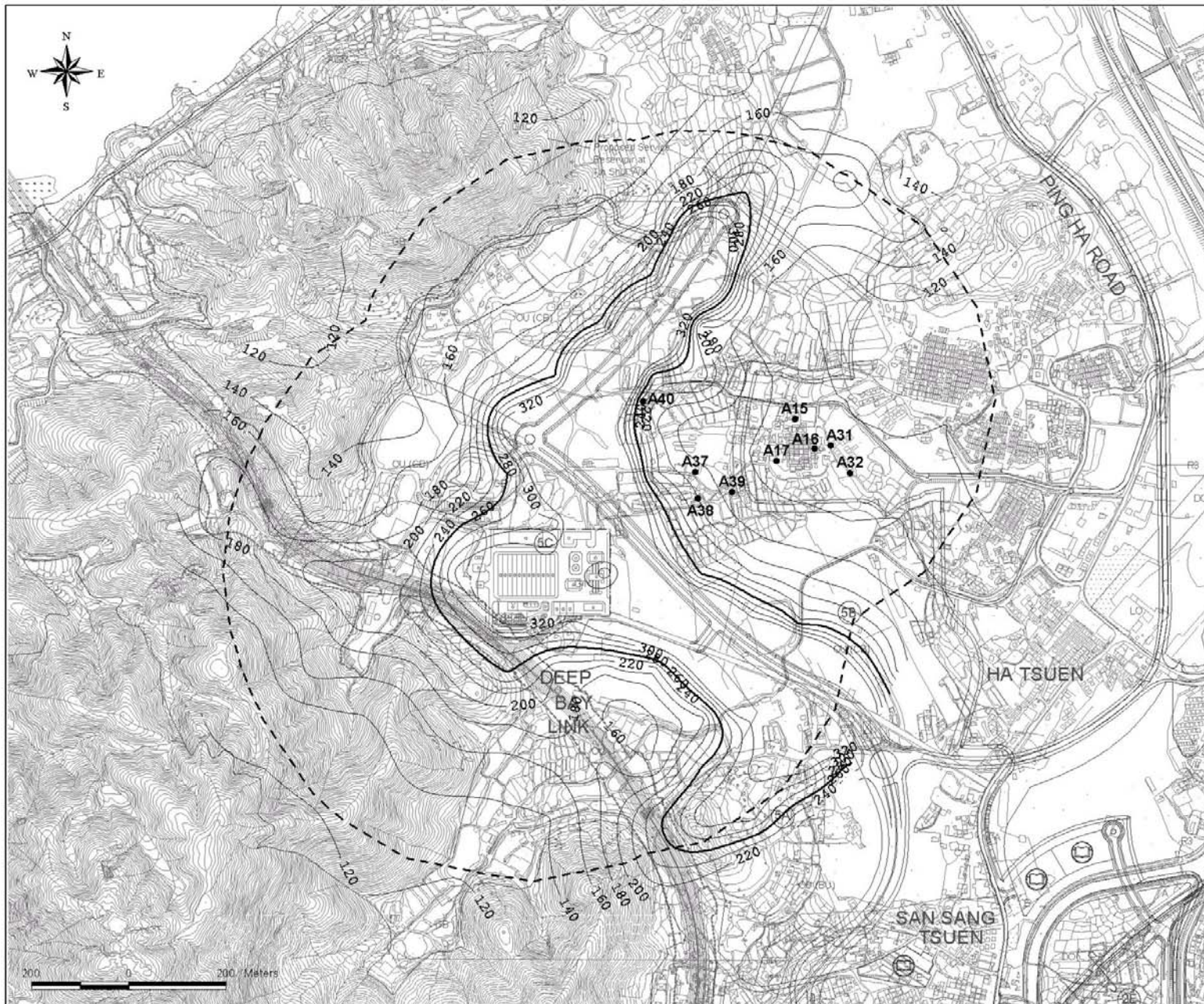
Figure 3.10 Predicted Worst-case Daily Average TSP Concentration Contours at 1.5m Above Ground for Mitigated Scenario around the Proposed Upgraded and Expanded San Wai STW
