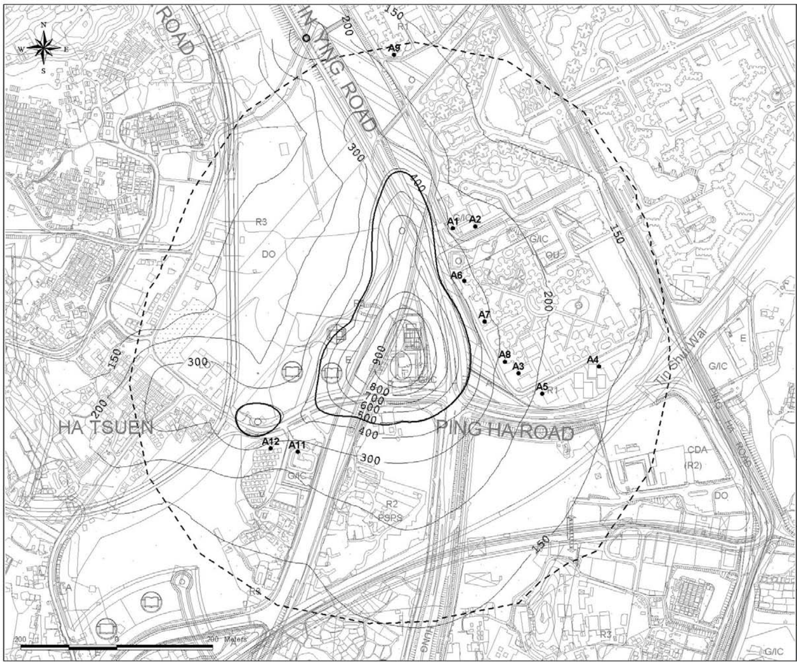
Figure 3.11 Predicted Worst-case Hourly Average TSP Concentration Contours at 1.5m Above Ground for Unmitigated Scenario around the Proposed Expanded Ha Tsuen PS
