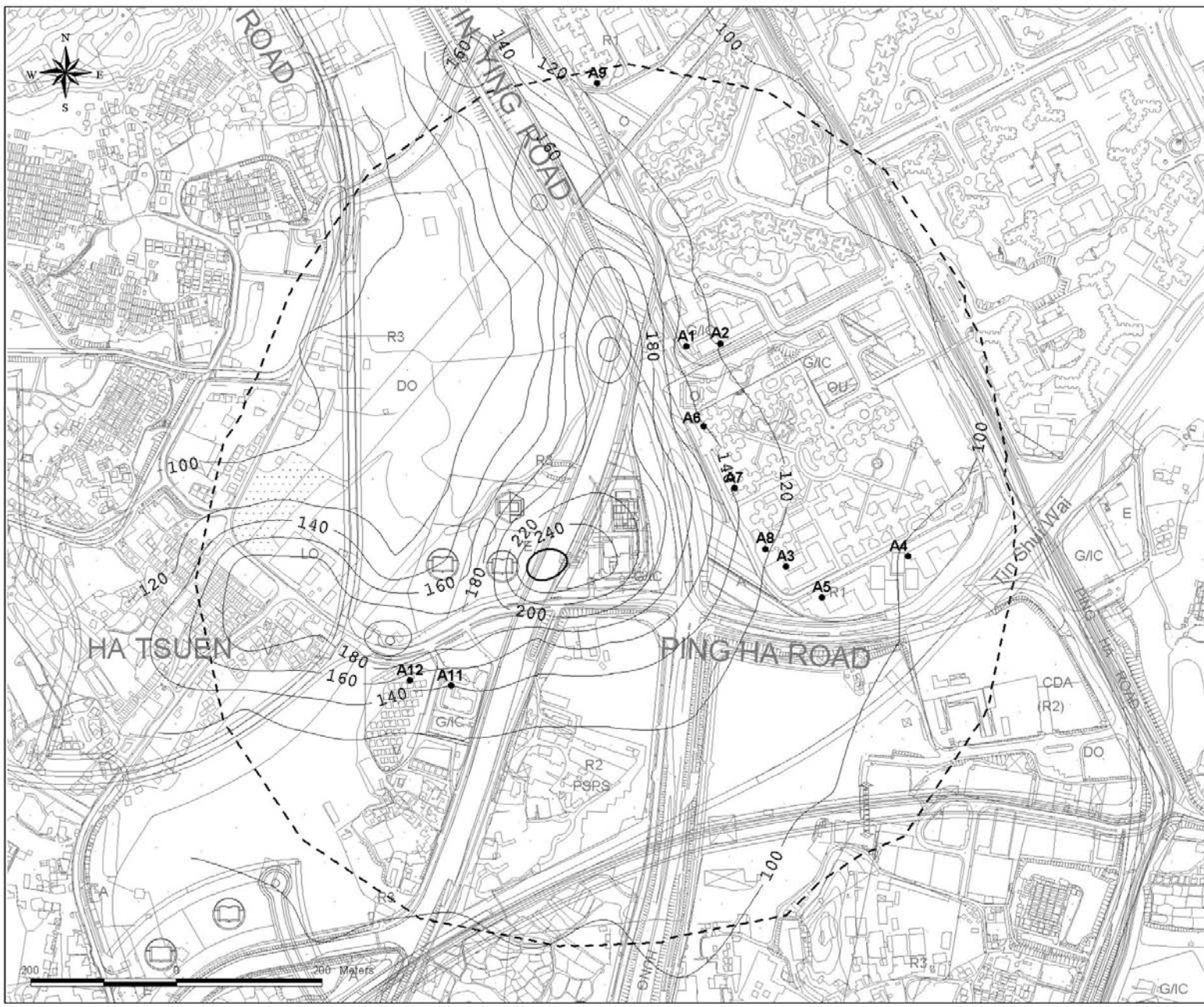
Figure 3.14 Predicted Worst-case Daily Average TSP Concentration Contours at 1.5m Above Ground for Mitigated Scenario around the Proposed Expanded Ha Tsuen PS
