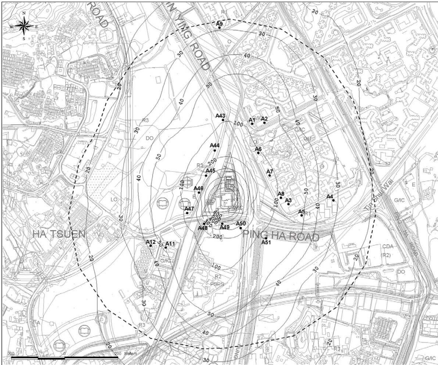
Figure 3.17 Predicted Worst-case 5-second Average Odour Levels at 1.5m above Ground for the Unmitigated Scenario around the Proposed Expanded Ha Tsuen PS
