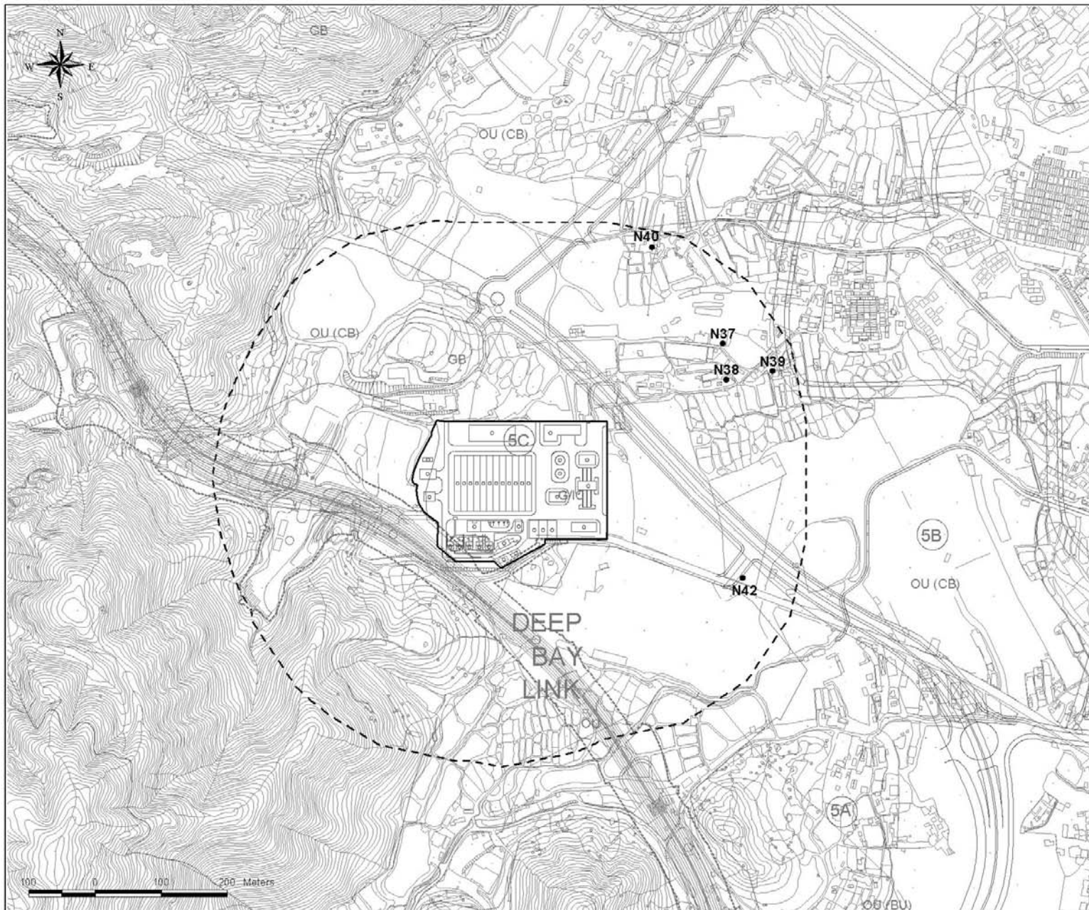
Figure 4.1 Assessment Area around the Proposed Expanded San Wai Sewage Treatment Works
