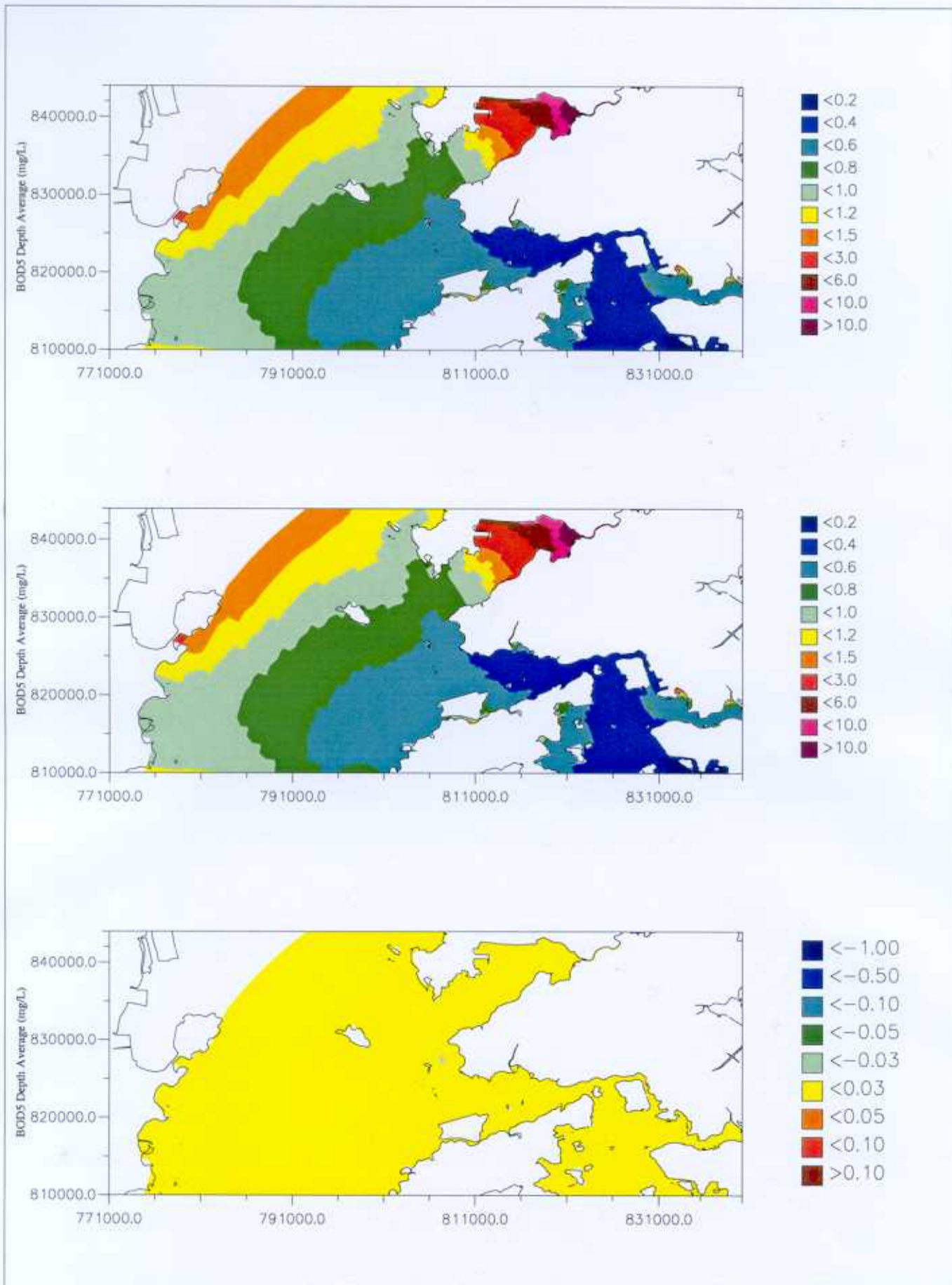
Upgrading and Expansion of San Wai STW and the Expansion of Ha Tsuen PS WQ Simulation – Comparison of BOD5 for Option 2 & 3 Upper: Option 2; Mid: Option 3; Lower: Absolute Difference (Opt 3 – Opt 2)
