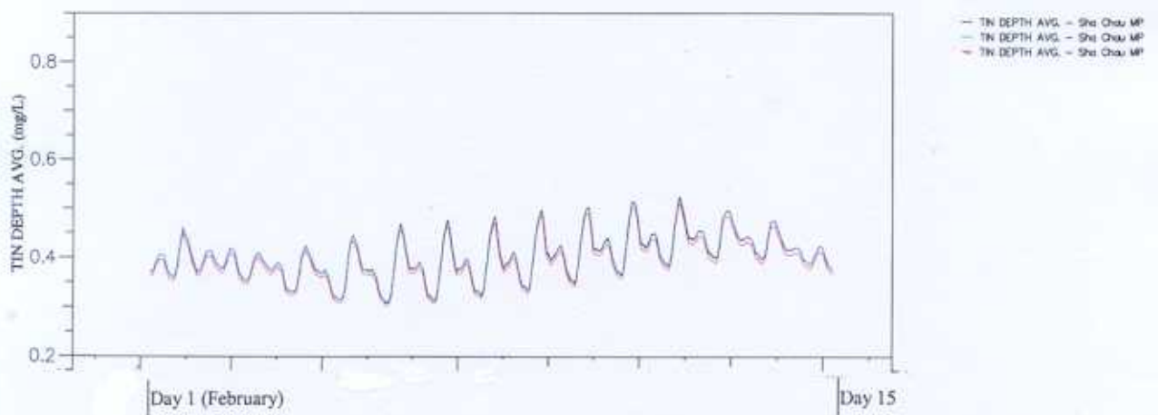
Upgrading and Expansion of San Wai STW and the Expansion of Ho Tsuen PS: Time Series Plot for TIN for Dry Season (Black: Baseline; Blue: Opt 3; Red: Opt 4) Upper: NM5; Mid: DM5; Lower: Sha Chau/Lung Kwu Chau Marine Park
