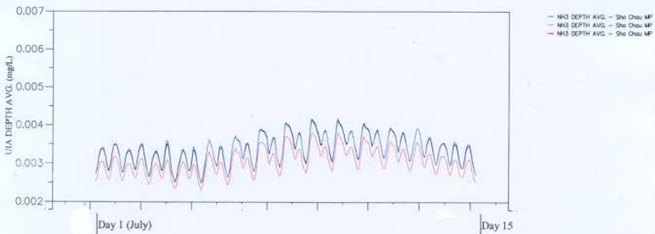
Upgrading and Expansion of San Wai STW and the Expansion of Ha Tsuen PS Time Series Plot for UIA for Wet Season (Black: Baseline; Blue: Opt 3; Red: Opt 4) Upper: NM5; Mid: DM5; Lower: Sho Chau/Lung Kwu Chau Marine Park
