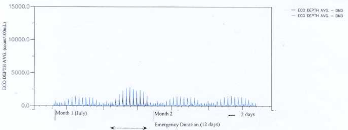
Upgrading and Expansion of San Wai STW and the Expansion of Ho Tsuen PS Time Series Plot for E.Coli with Emergency Discharge at Tin Shui Wai - Wet Season (1) Upper: DM1; Mid: DM 2; Lower: DM3 (Black: Opt 2 Normal; Blue: Sanwai Raw Sewage)
