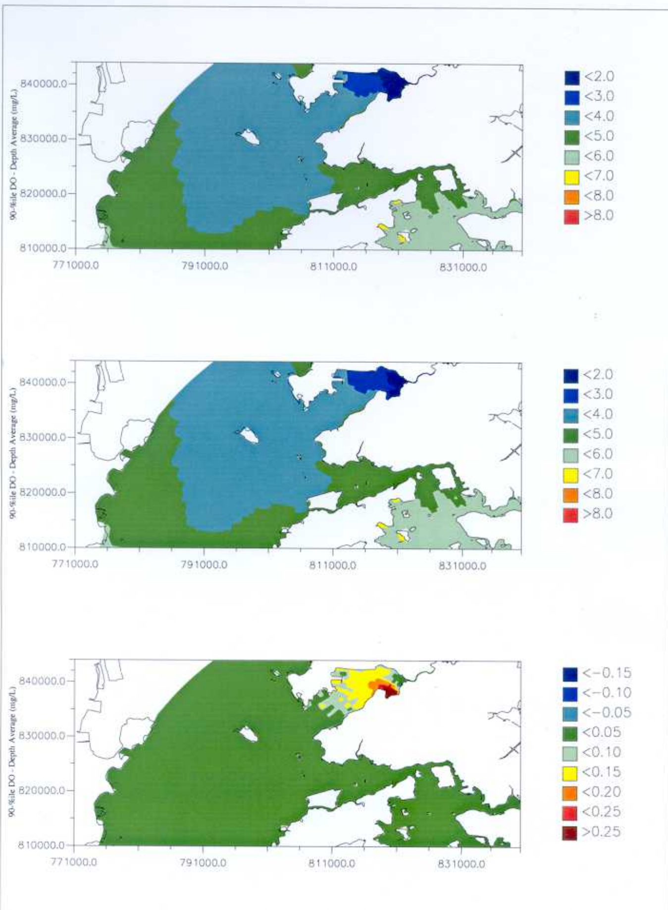
Upgrading and Expansion of San Wai STW and the Expansion of Ha Tsuen PS WQ Simulation - Comparison of 90-%ile DO Depth-Average for Baseline & Option 1 Upper: Baseline; Mid: Option 1; Lower: Absolute Difference (Option 1 - Baseline) November 2002 Figure 5.2 MWH
