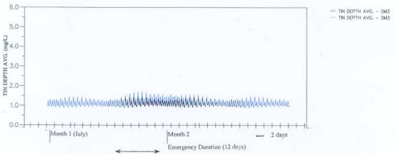
Upgrading and Expansion of San Wai STW and the Expansion of Ho Tsuen PS Time Series Plot for TIN with Emergency Discharge at Tin Shui Wai - Wet Season (1) Upper: DM1; Mid: DM2; Lower: DM3 (Black: Opt. 2 Normal; Blue: Sanwai Raw Sewage)
