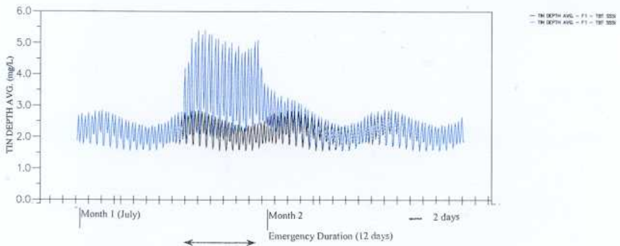
Upgrading and Expansion of San Wai STW and the Expansion of Ho Tsuen PS Time Series Plot for TIN with Emergency Discharge at Tin Shui Wai - Wet Season (2) Upper: Pak Nai; Mid: Mai Po; Lower: Tsim Bei Tsui (Black: Opt 2 Normal; Blue: Sanwai Raw Sewage)
