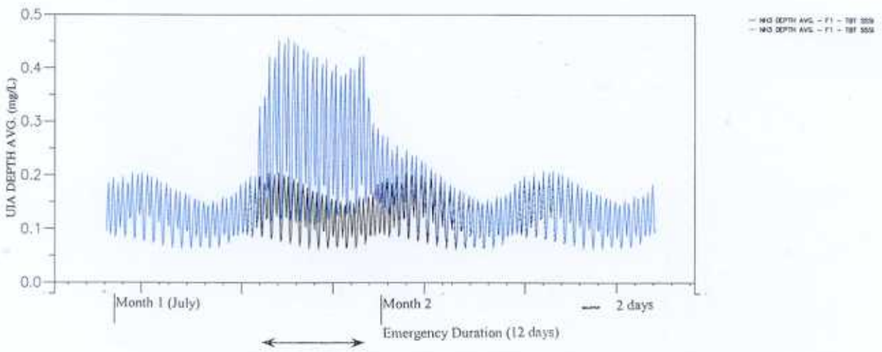
Upgrading and Expansion of San Wai STW and the Expansion of Ho Tsuen PS Time Series Plot for UTA with Emergency Discharge at Tin Shui Wai – Wet Season (2) Upper: Pak Nai; Mid: Mai Po; Lower: Tsim Bei Tsui (Black: Opt. 2 Normal; Blue: Sanwai Raw Sewage)
