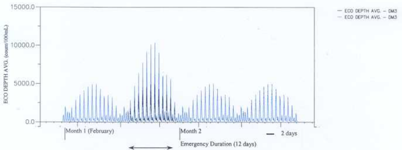
Upgrading and Expansion of San Wai STW and the Expansion of Ha Tsuen PS Time Series Plot for E.Coli with Emergency Discharge at Tin Shui Wai - Dry Season (1) Upper: DM1; Mid: DM 2; Lower: DM3 (Black: Opt 2 Normal; Blue: Sanwai Raw Sewage)
