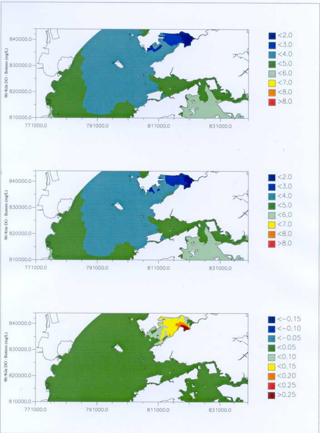
Upgrading and Expansion of San Wai STW and the Expansion of Ha Tsuen PS WQ Simulation - Comparison of 90-%ile DO Bottom for Baseline & Option 1 Upper: Baseline; Mid: Option 1; Lower: Absolute Difference (Option 1- Baseline) November 2002 Figure 5.3 MWH
