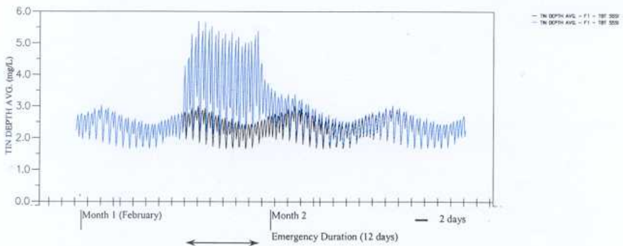
Upgrading and Expansion of San Wai STW and the Expansion of Ha Tsuen PS Time Series Plot for TIN with Emergency Discharge at Tin Shui Wai - Dry Season (2) Upper: Pak Nai; Mid: Mai Po; Lower: Tsim Bei Tsui (Black: Opt 2 Normal; Blue: Sanwai Row Sewage)
