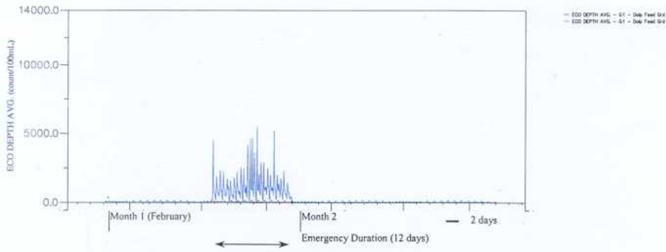
Upgrading and Expansion of San Wai STW and the Expansion of Ha Tsuen PS Time Series Plot for Station G1 with Emergency Discharge at Urmston Rd. - Dry Season (2) Upper: TIN; Middle: UIA; Lower: E.Coli (Black: Option 2 Normal; Blue: San Wai Raw Sewage) November 2002 Figure 5.38 MWH
