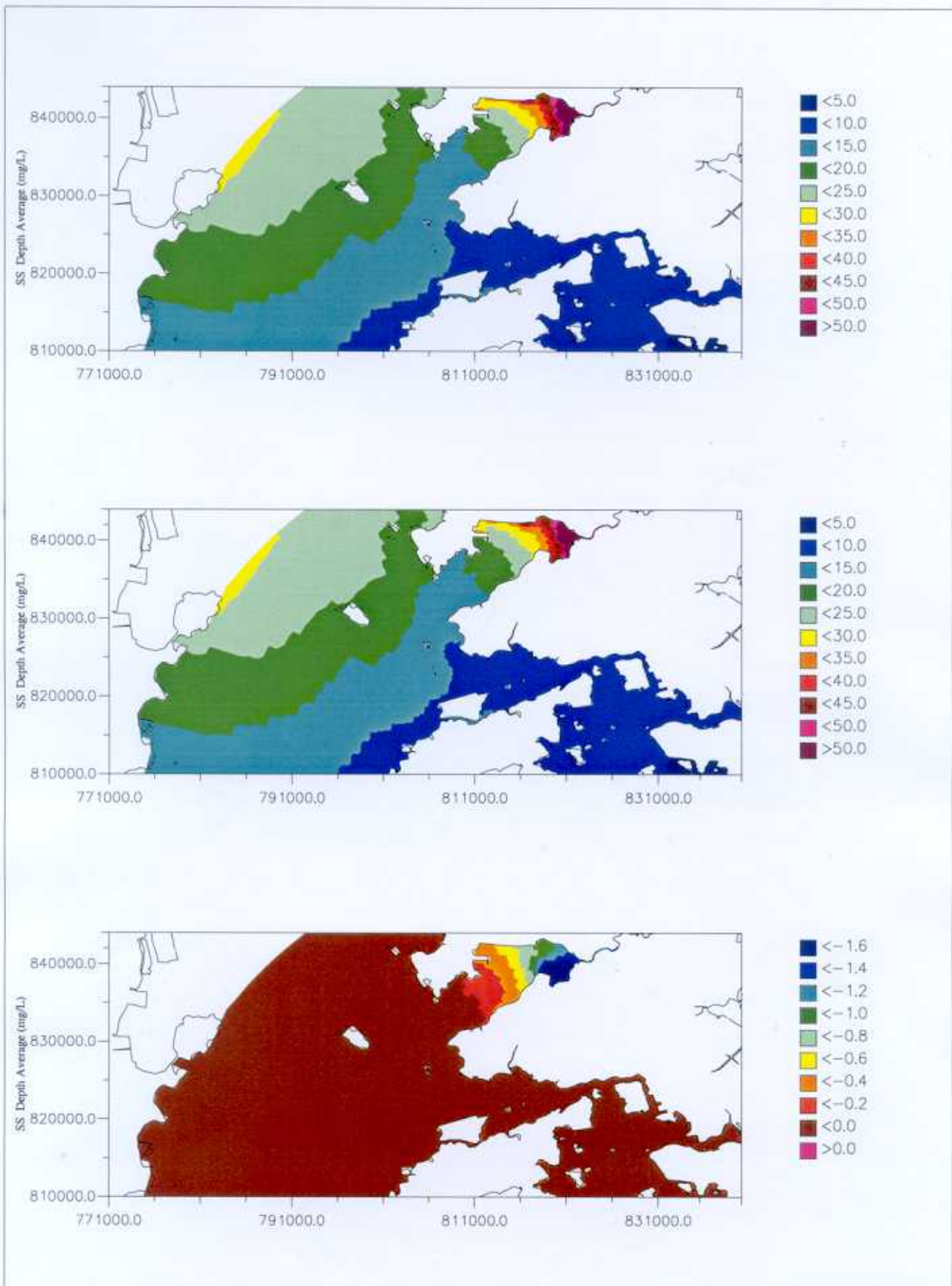
Upgrading and Expansion of San Wai STW and the Expansion of Ho Tsuen PS WQ Simulation – Comparison of SS for Baseline & Option 1 Upper: Baseline; Mid: Option 1; Lower: Absolute Difference (Option 1 – Baseline)
