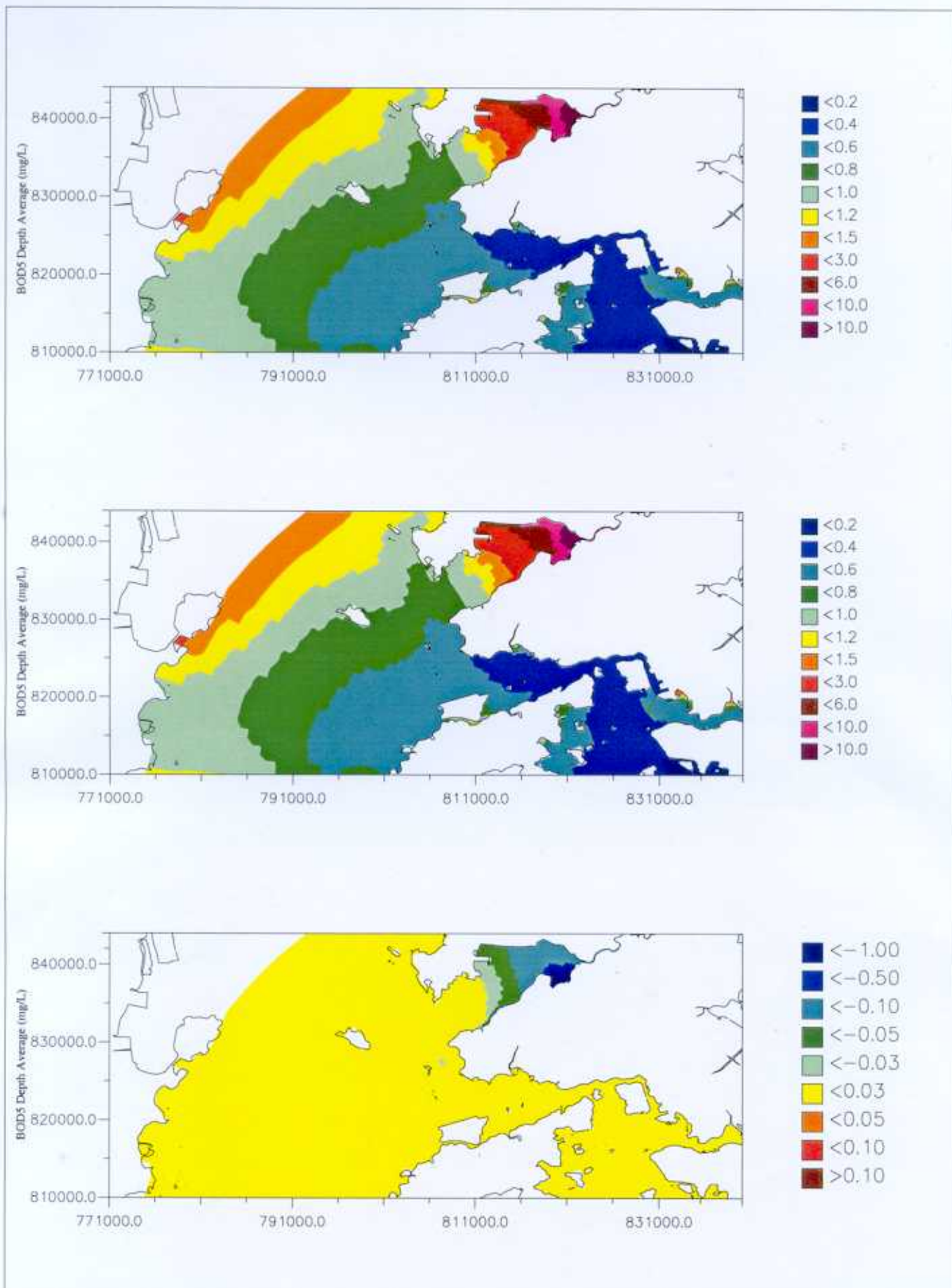
Upgrading and Expansion of San Wai STW and the Expansion of Ha Tsuen PS WQ Simulation – Comparison of BOD5 for Baseline & Option 1 Upper: Baseline; Mid: Option 1; Lower: Absolute Difference (Option 1 – Baseline)
